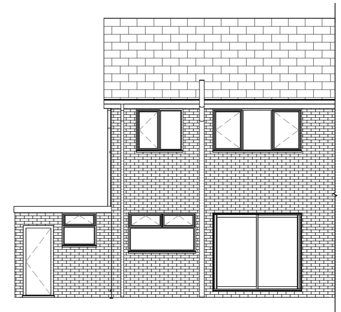
3 Rear Elevation 1 : 100
