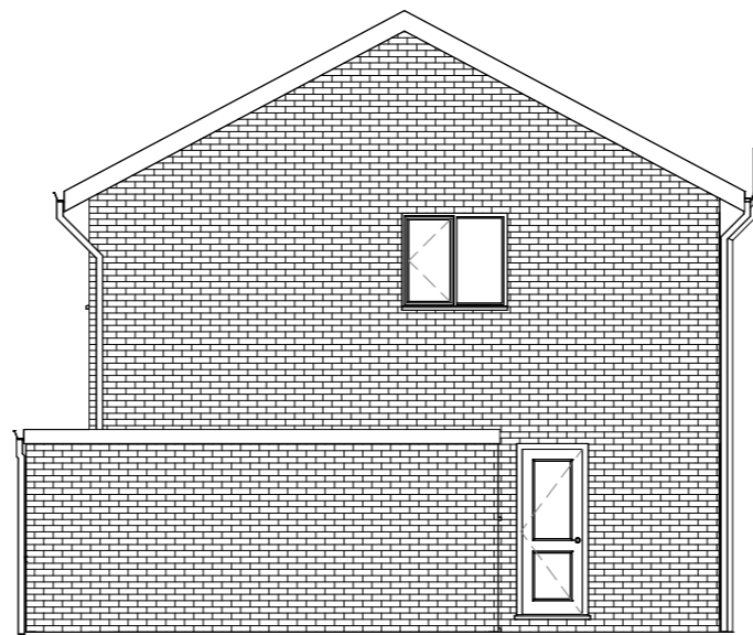
2 Gable Elevation 1 : 100
