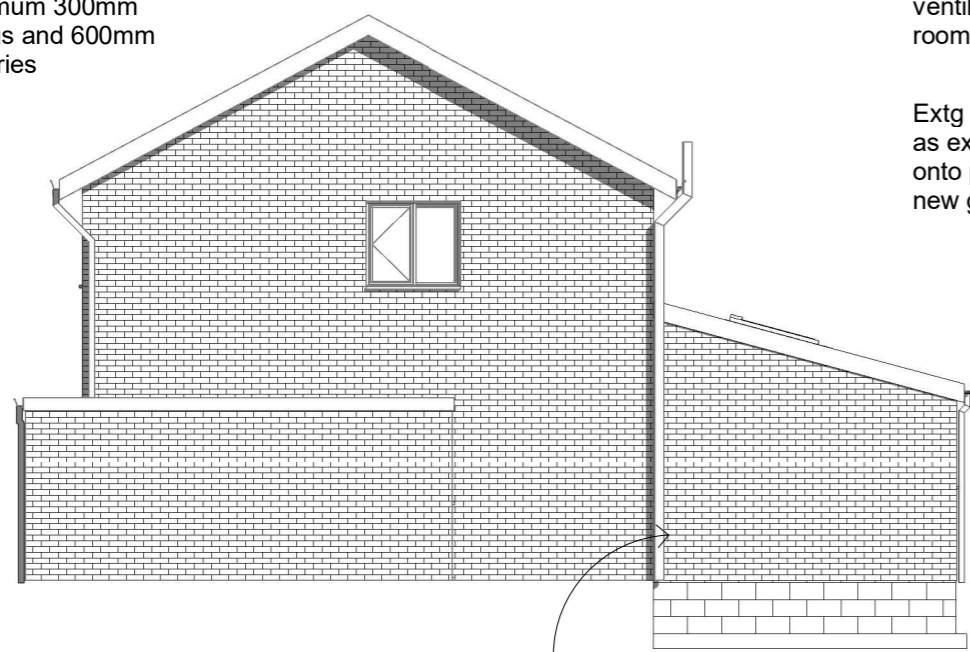
1 Gable Elevation 1 : 100
