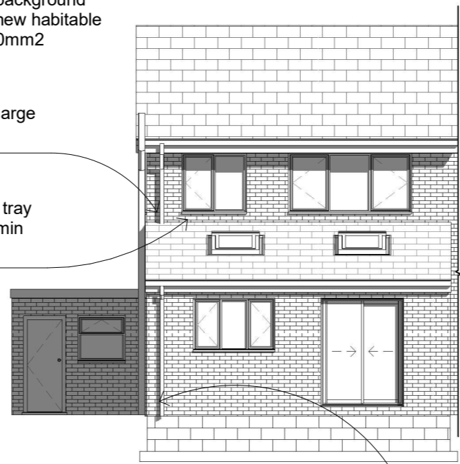
2 Rear Elevation 1 : 100
