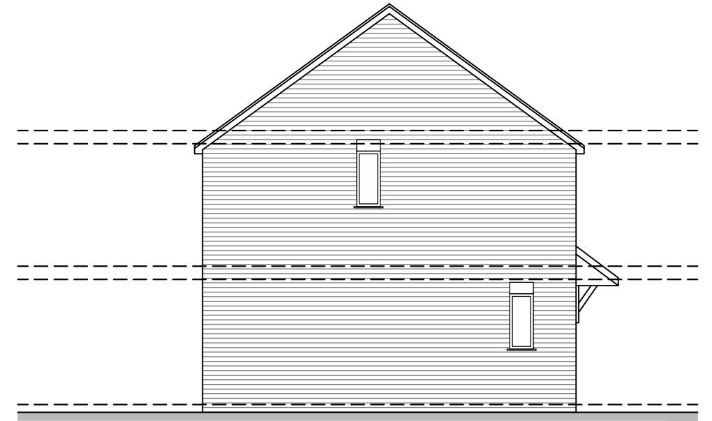
SIDE ELEVATION 1:100
