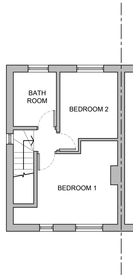
FIRST FLOOR PLAN 1:100
