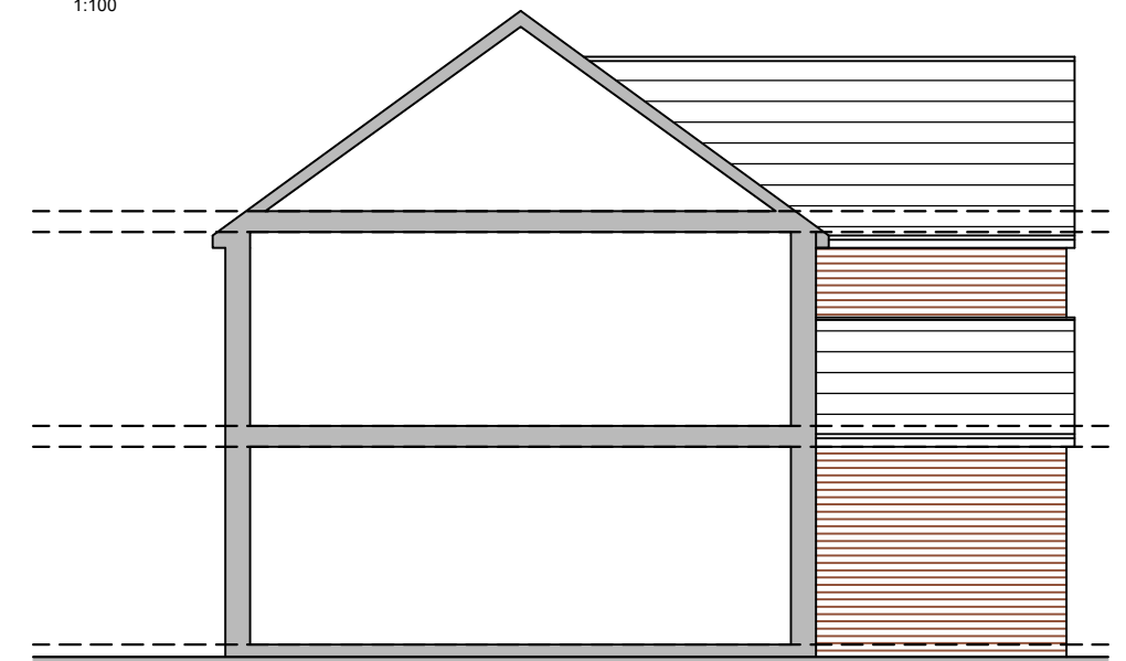
SIDE ELEVATION 1:100
