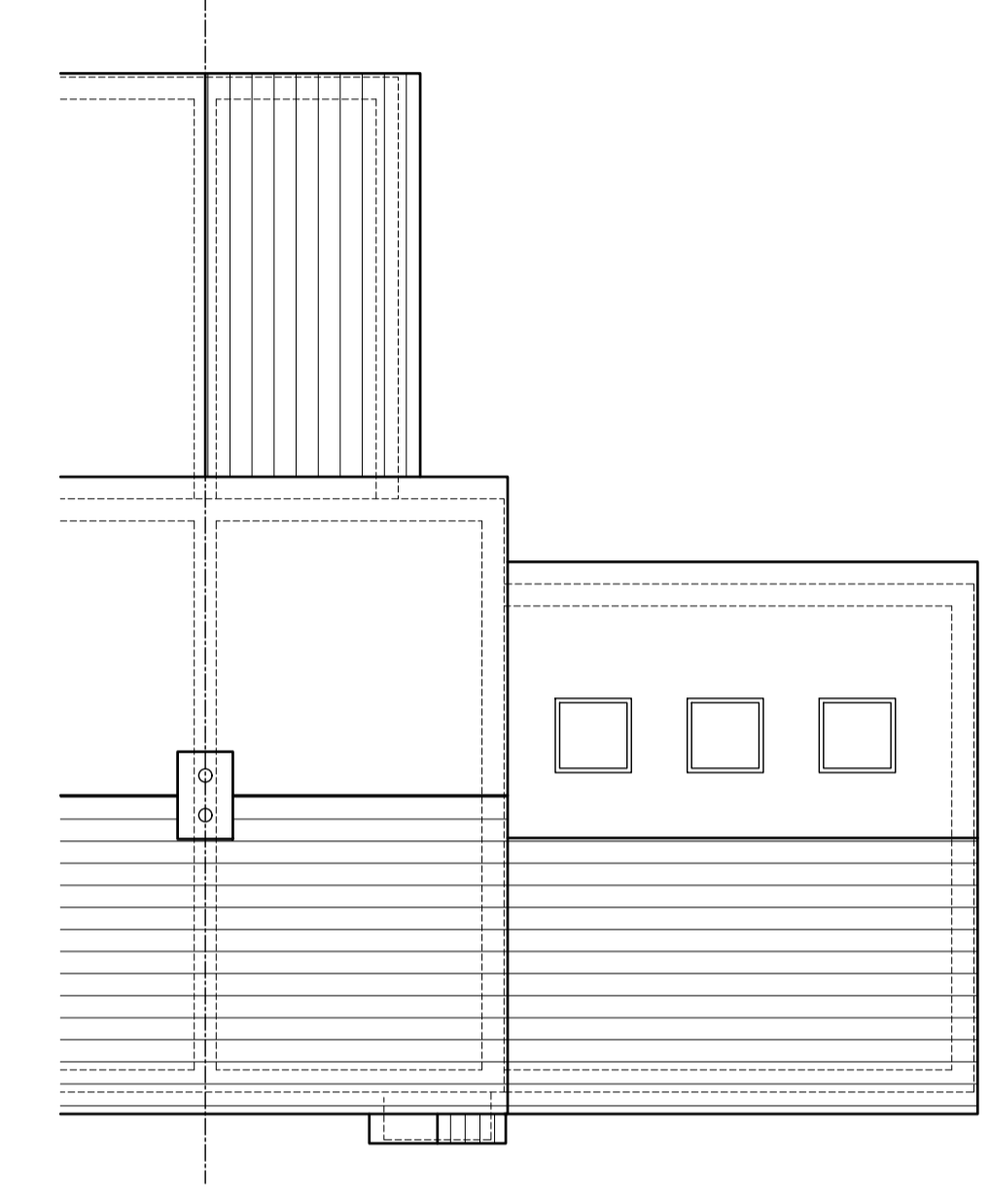
EXISTING ROOF
