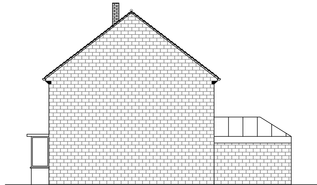
Proposed Right Elevations
