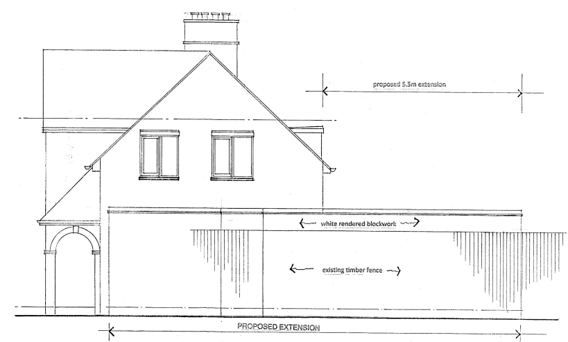
SIDE ELEVATION (east)
