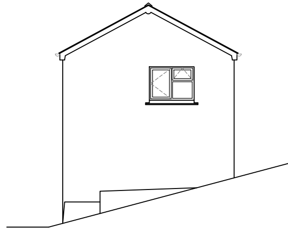
South Elevation
