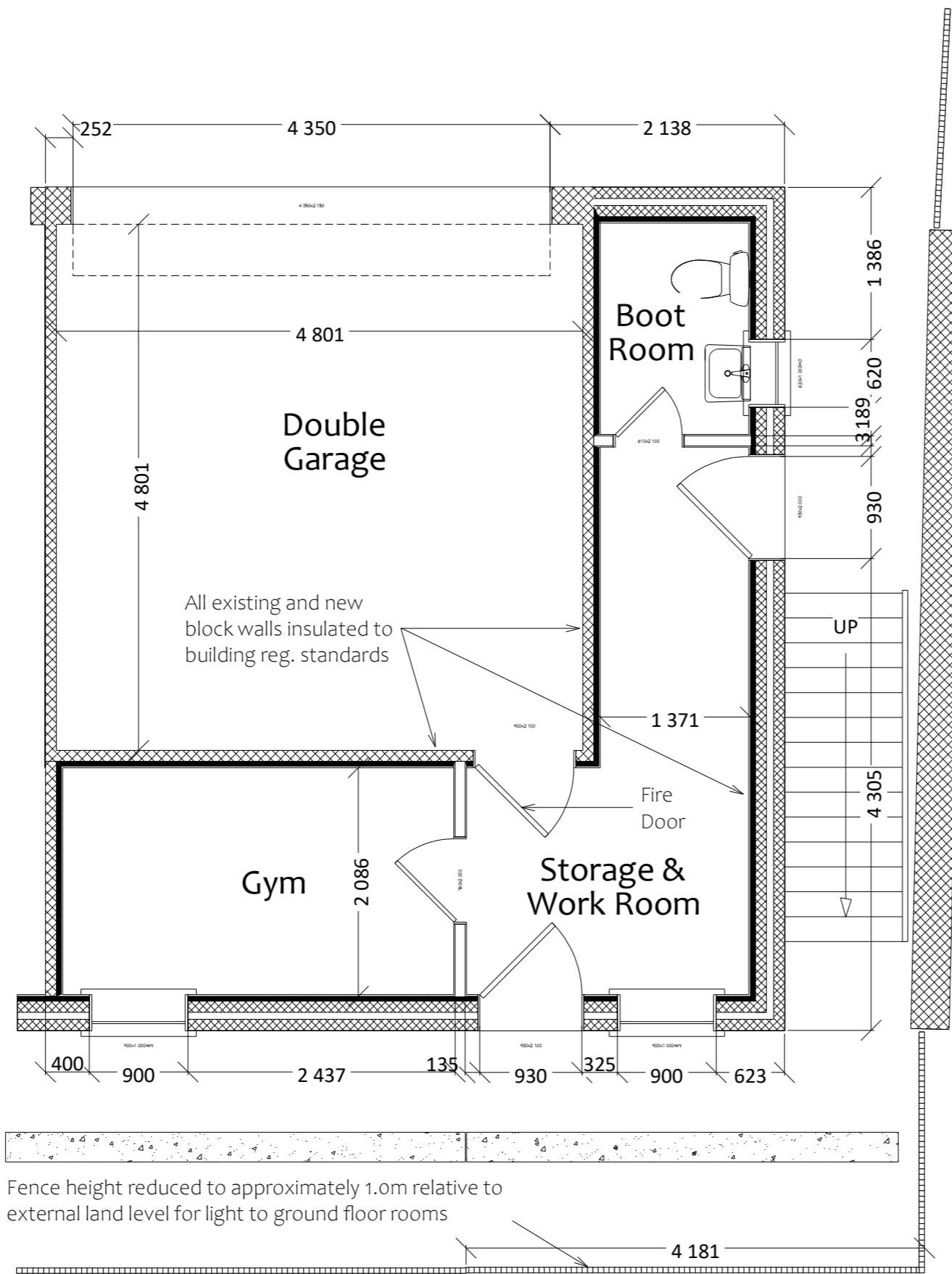
FP-03 Proposed Ground Floor Plan as per PA21-04432
