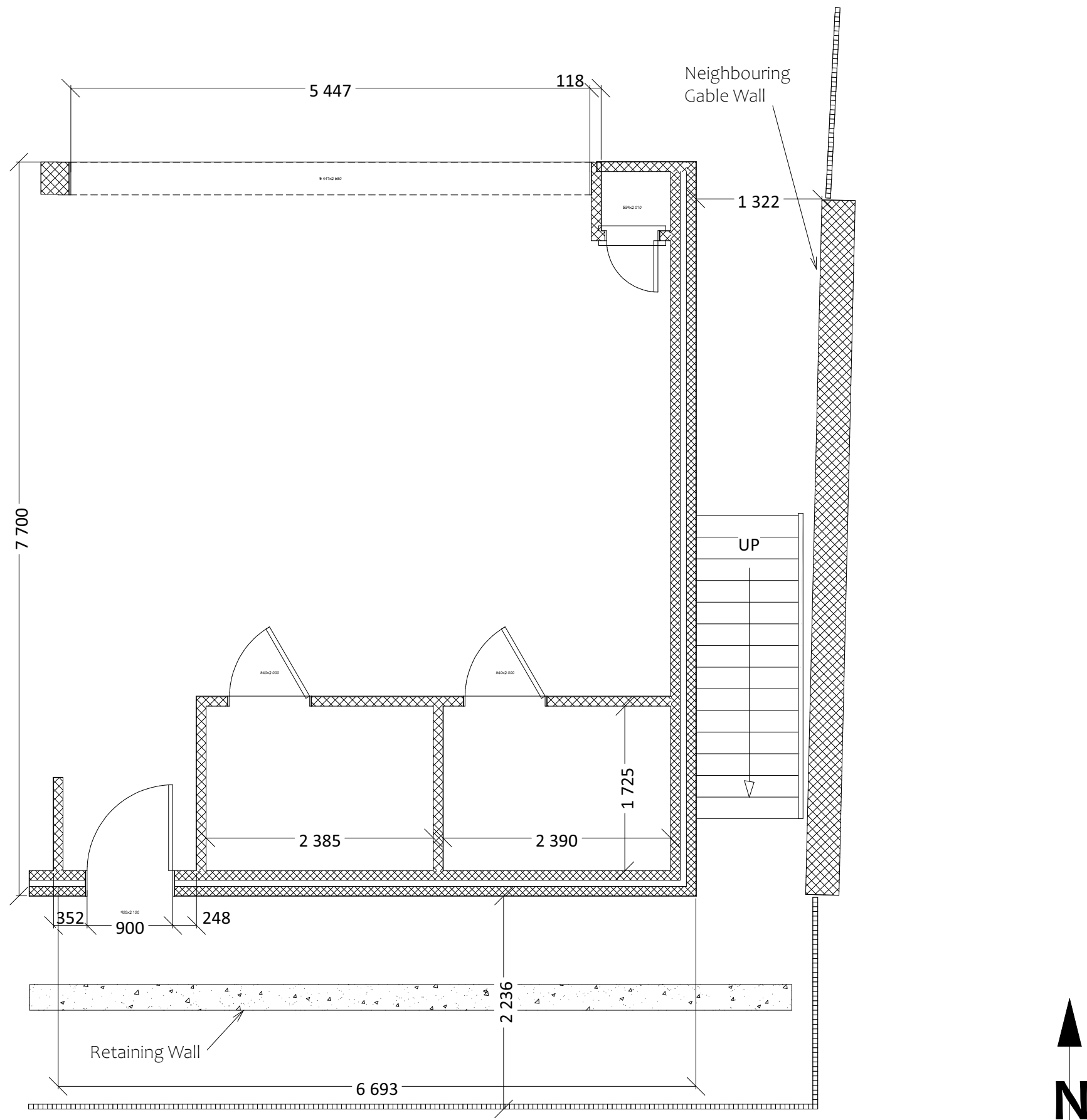
FP-01 Existing Ground Floor Plan
