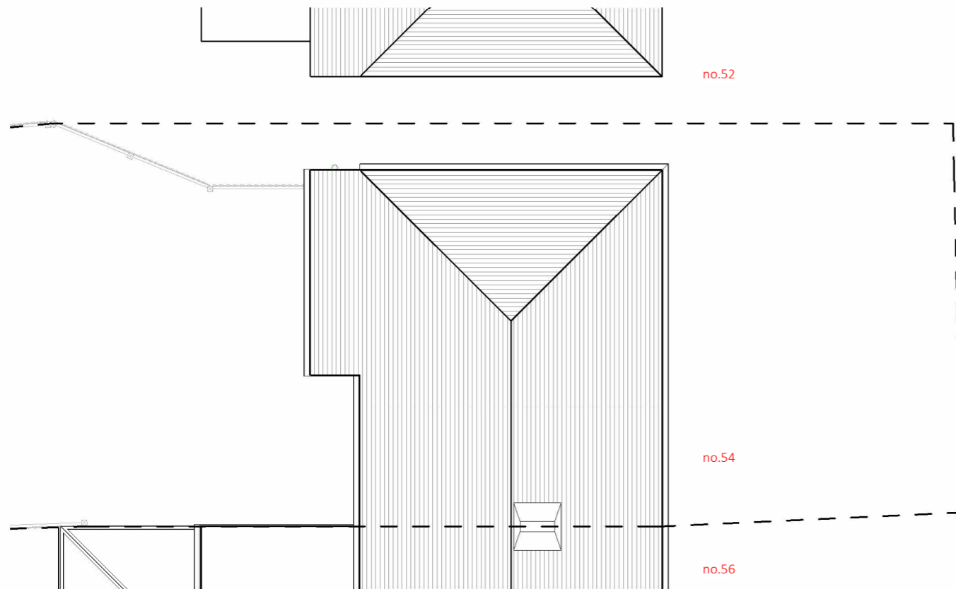
3 P02 P5.0 Roof Plan as existing 1:100
