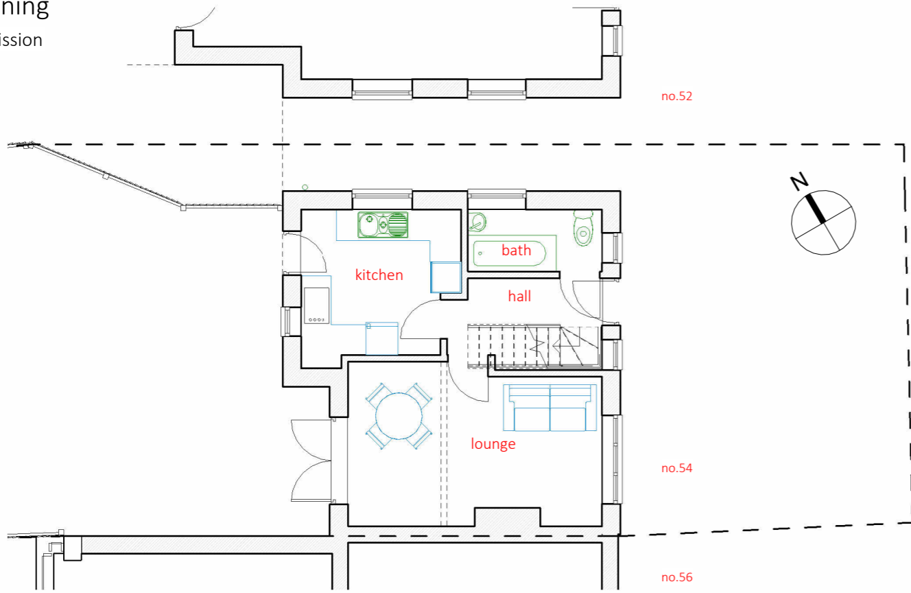
1 P02 P3.0 Ground floor as existing 1:100
