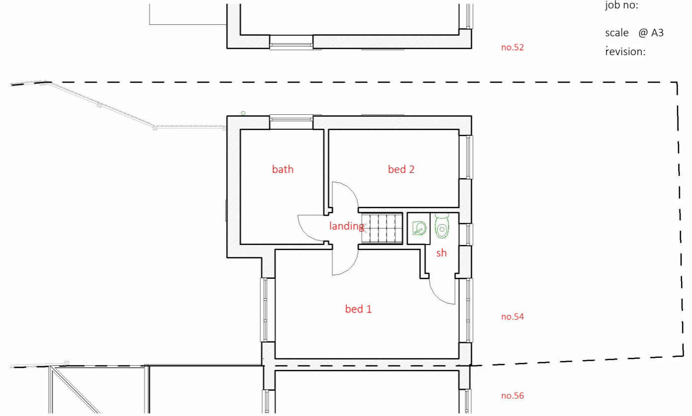
2 P02 P4.0 First Floor as existing 1:100
