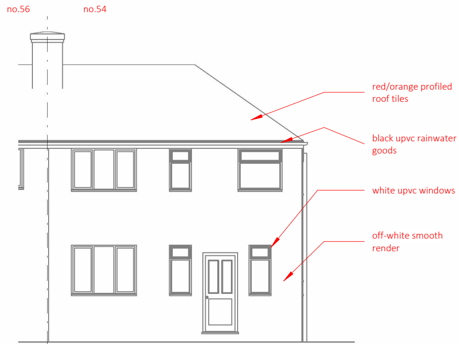
1 P05 south east elevation - proposed 1 : 100
