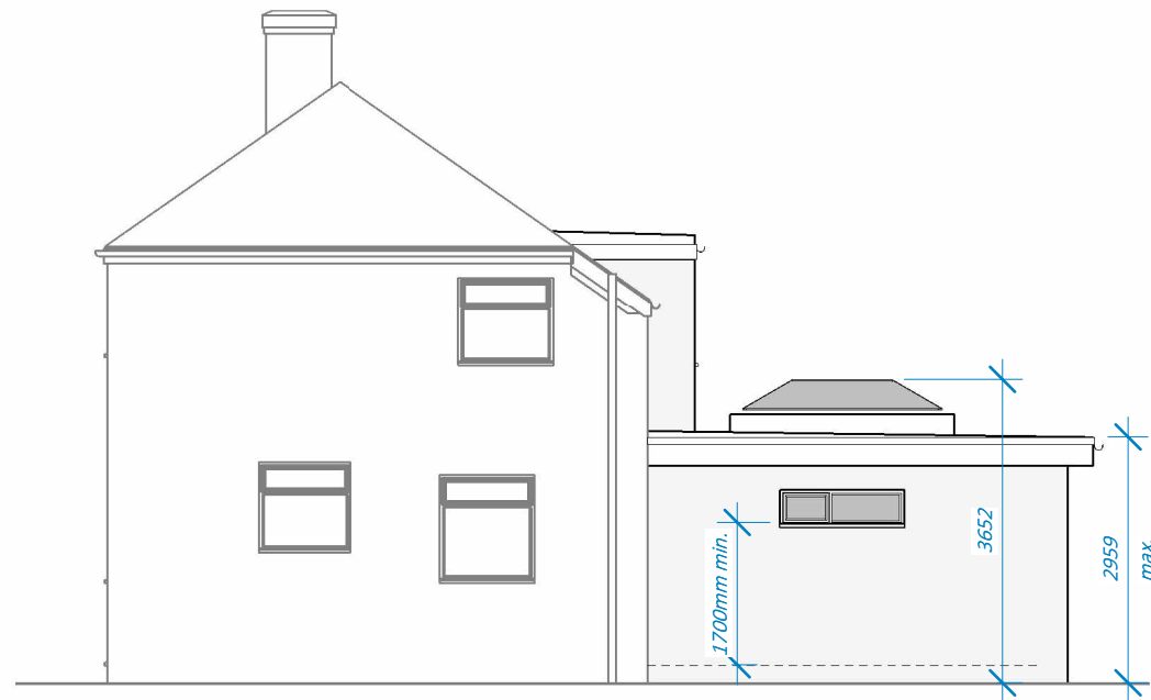
2 P05 north east elevation - proposed 1 : 100
