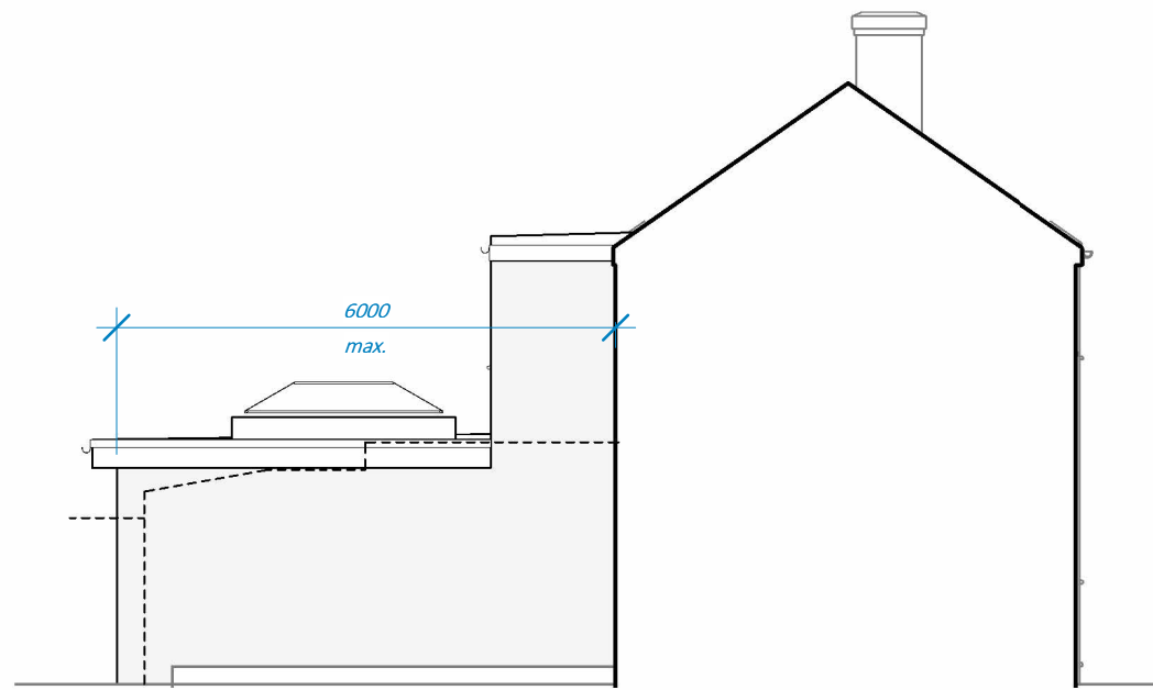
3 P05 south west elevation - proposed 1 : 100
