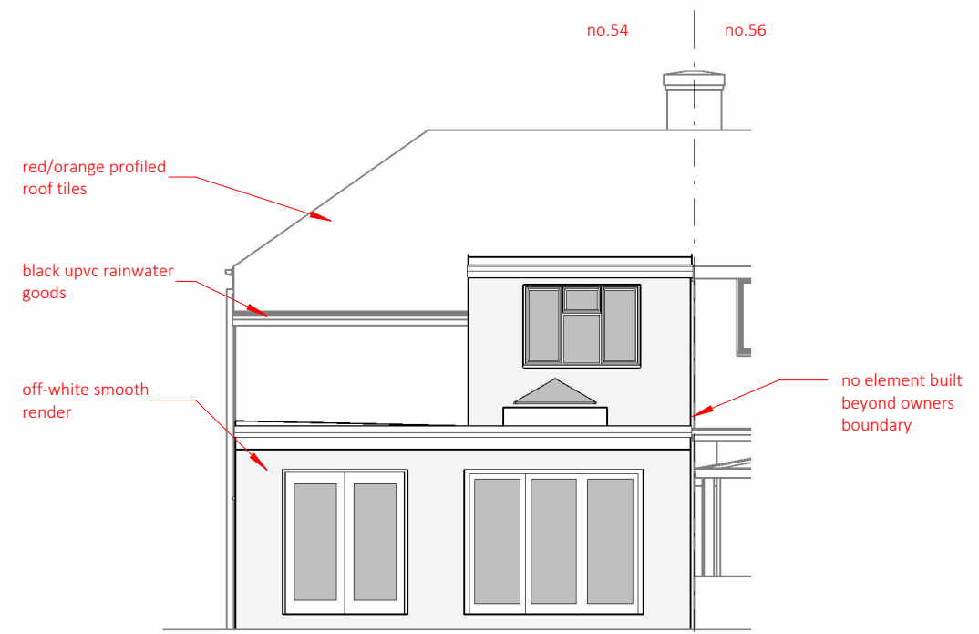
4 P05 north west elevation - proposed 1 : 100
