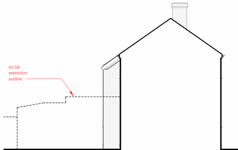
3 south west elevation - existing P03 1 : 100
