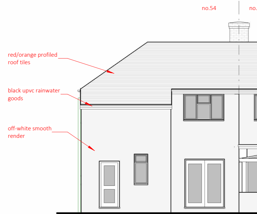
4 north west elevation - existing P03 1 : 100
