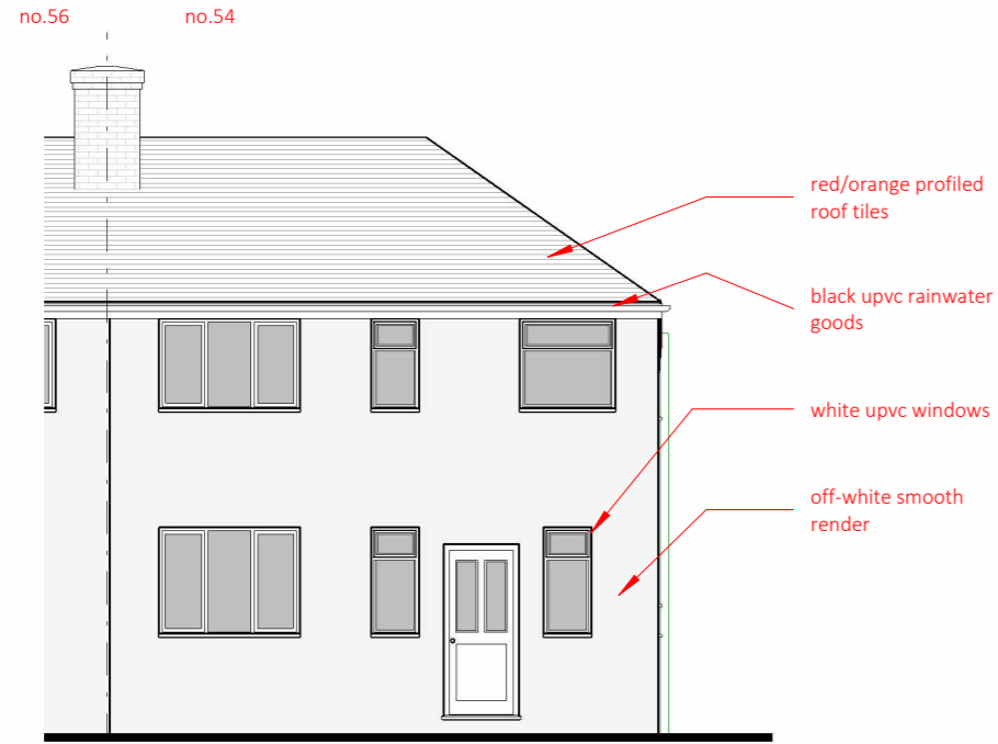
1 south east elevation - existing P03 1 : 100
