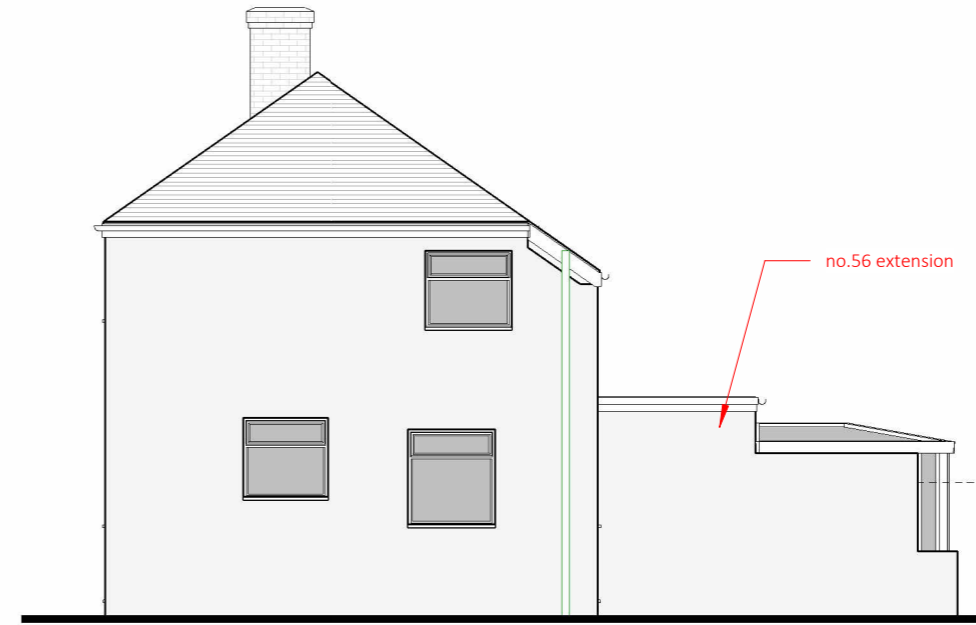
2 north east elevation - existing P03 1 : 100
