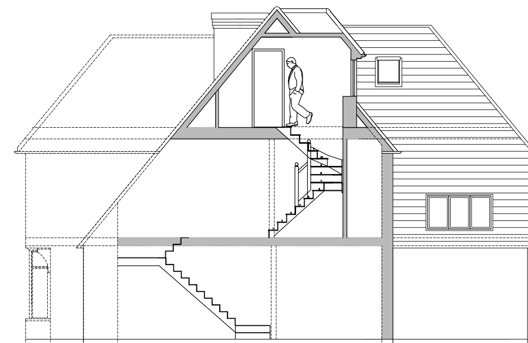
Section
