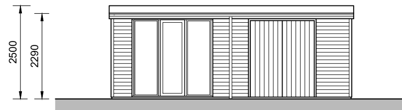
Front Elevation
