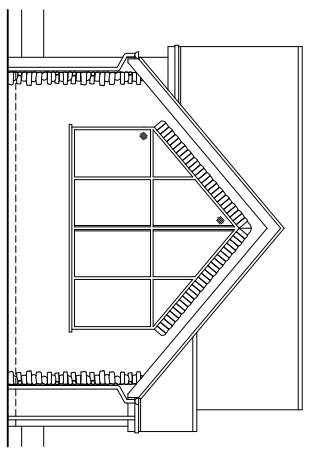
PROPOSED SIDE ELEVATION SCALE 1/50
