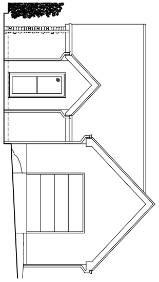
PROPOSED FRONT ELEVATION SCALE 1/50
