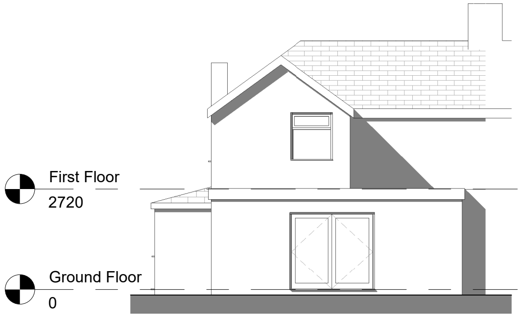
Rear Elevation 1 : 100
