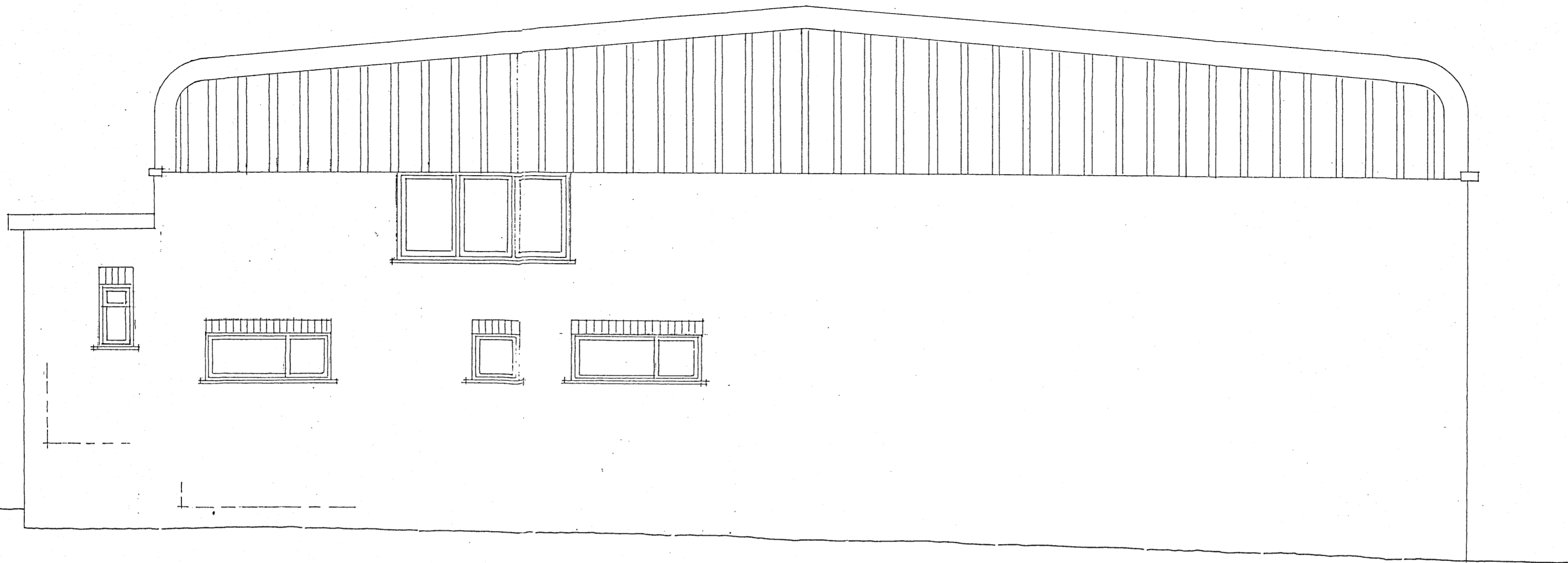
SIDE ELEVATION (WEST) ~ AS EXISTING
