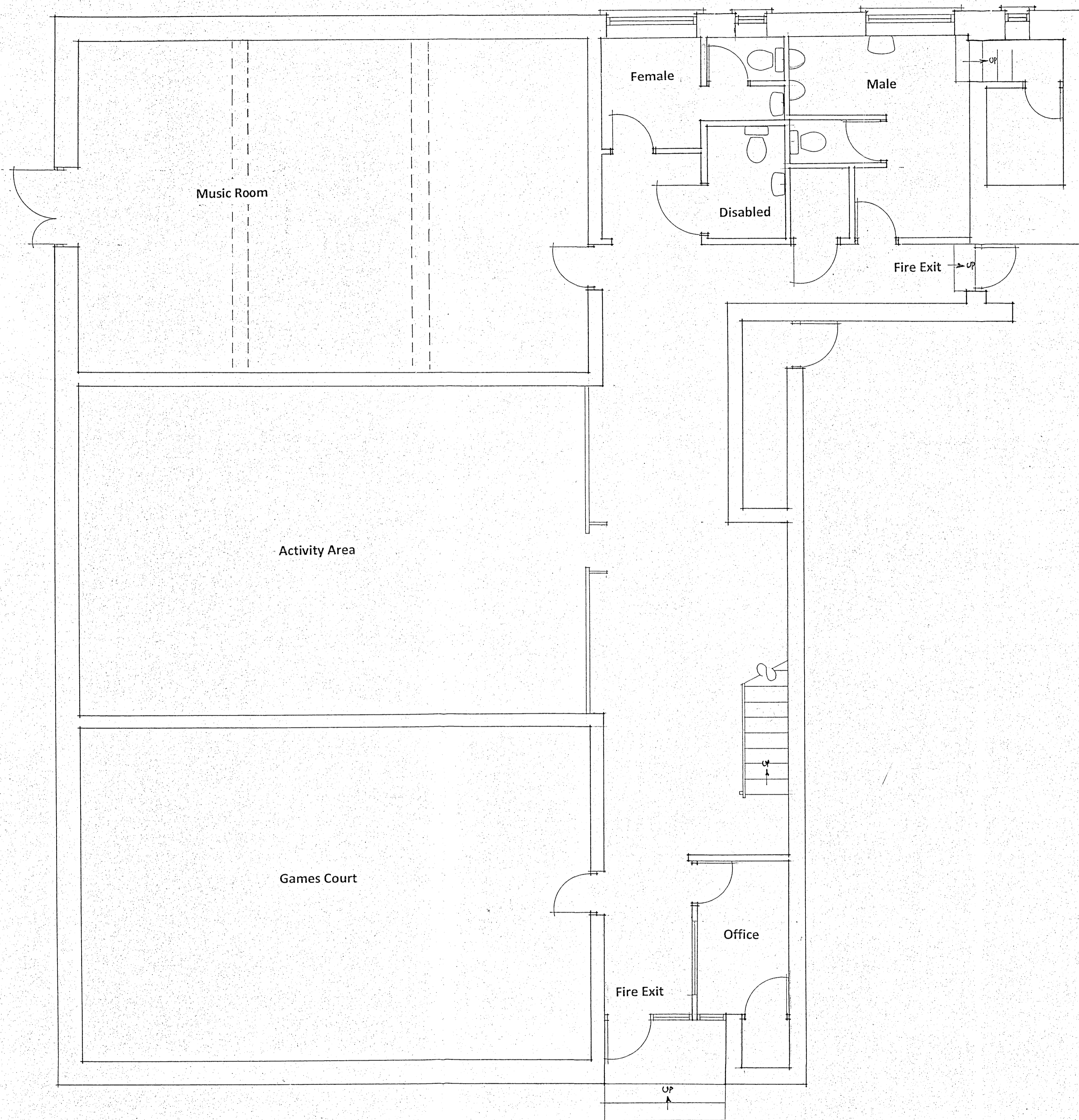
GROUND FLOOR PLAN ~ AS EXISTING
