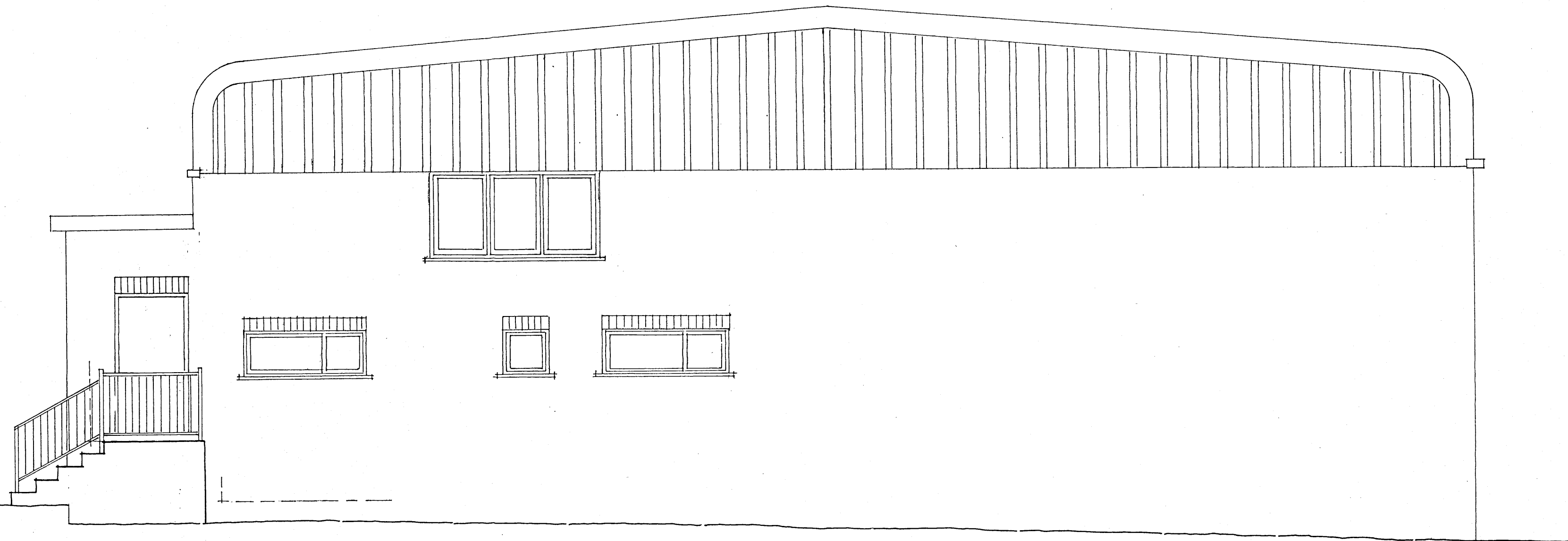
SIDE ELEVATION (WEST) ~ AS PROPOSED
