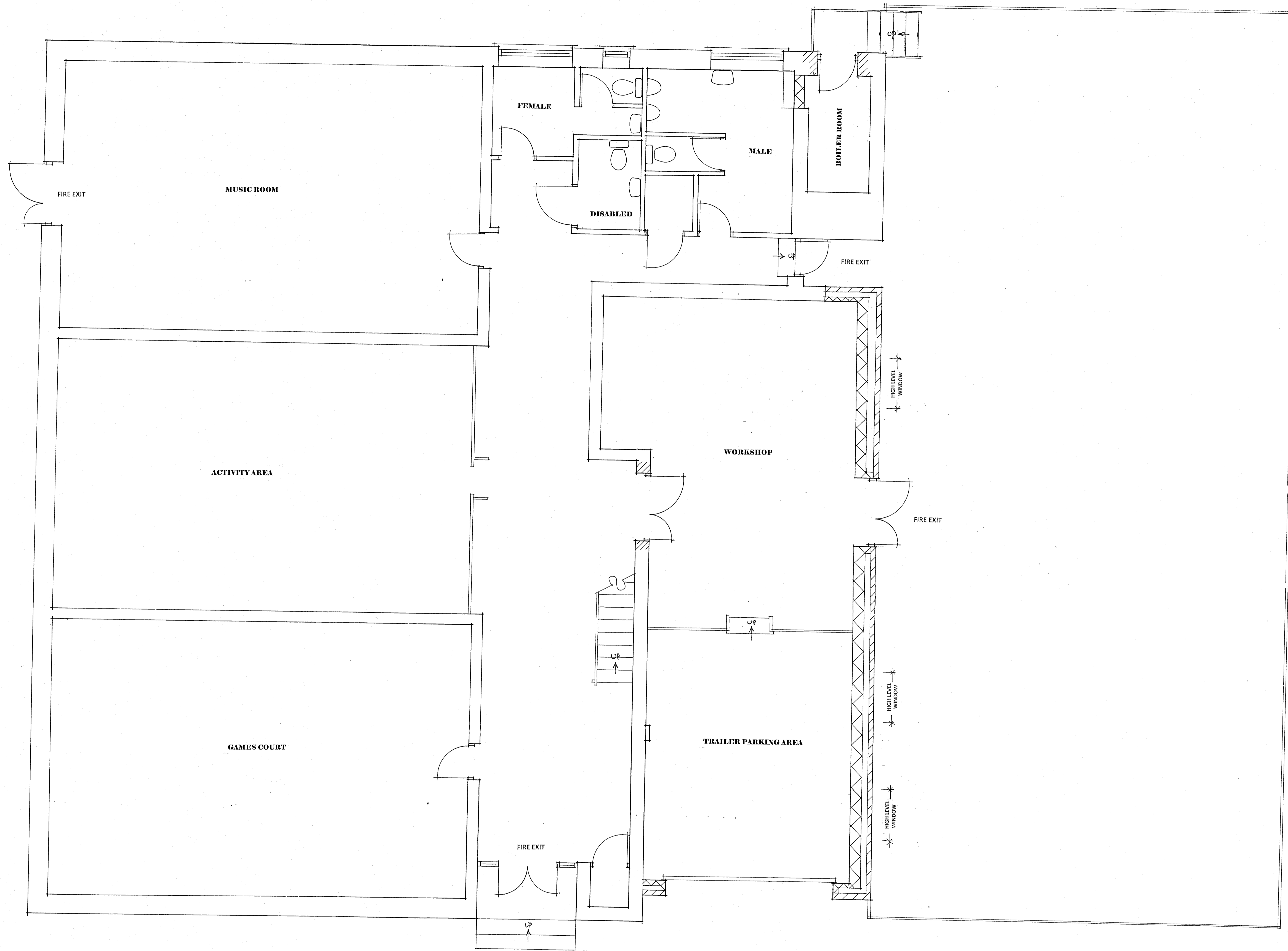
GROUND FLOOR PLAN ~ AS PROPOSED
