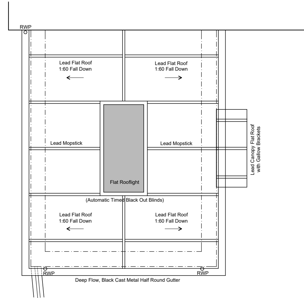
Proposed Extension Roof Plan 1:50
