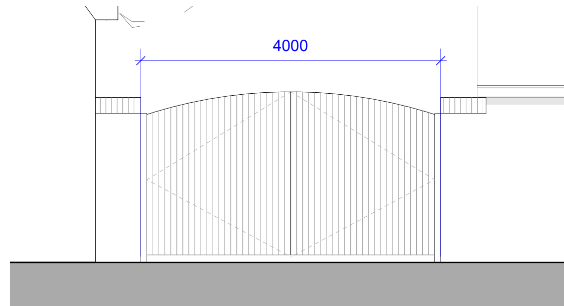
PROPOSED ENTRANCE GATE: ELEVATION 1:50
