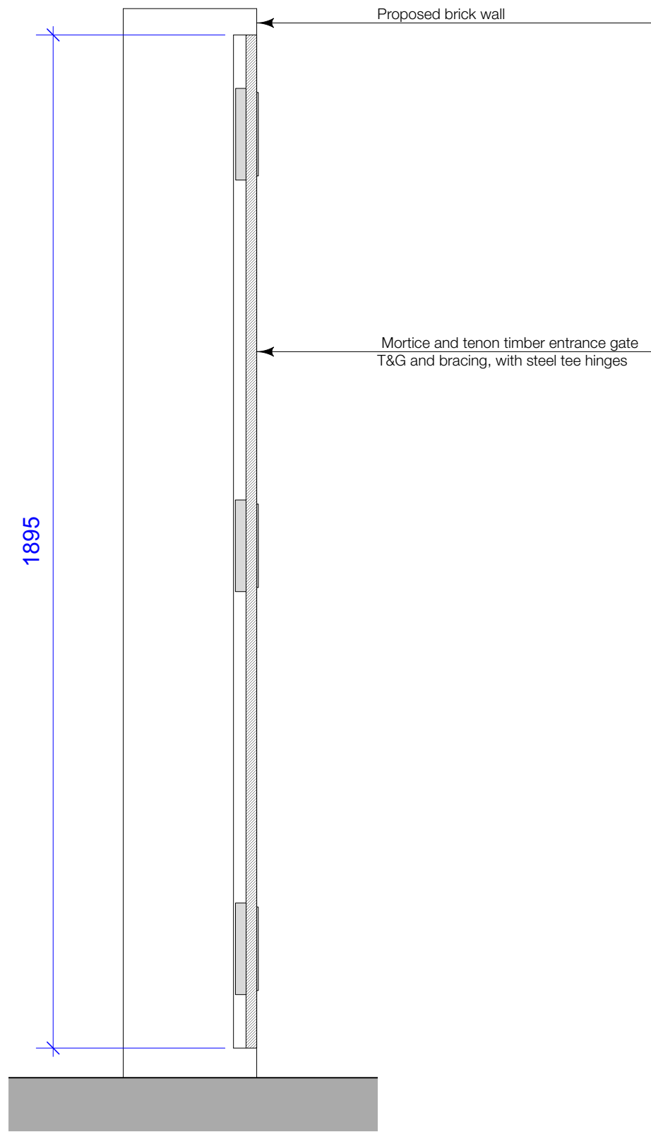
PROPOSED ENTRANCE GATE: JOINERY DETAIL 1:10
