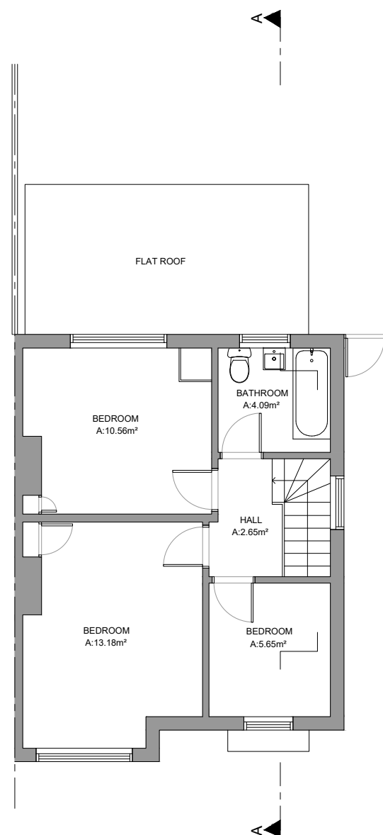
Existing First Floor Plan GIA: 40.92m 2
