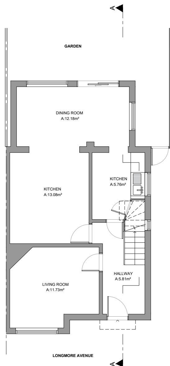
Existing Ground Floor Plan GIA: 54.36m 2
