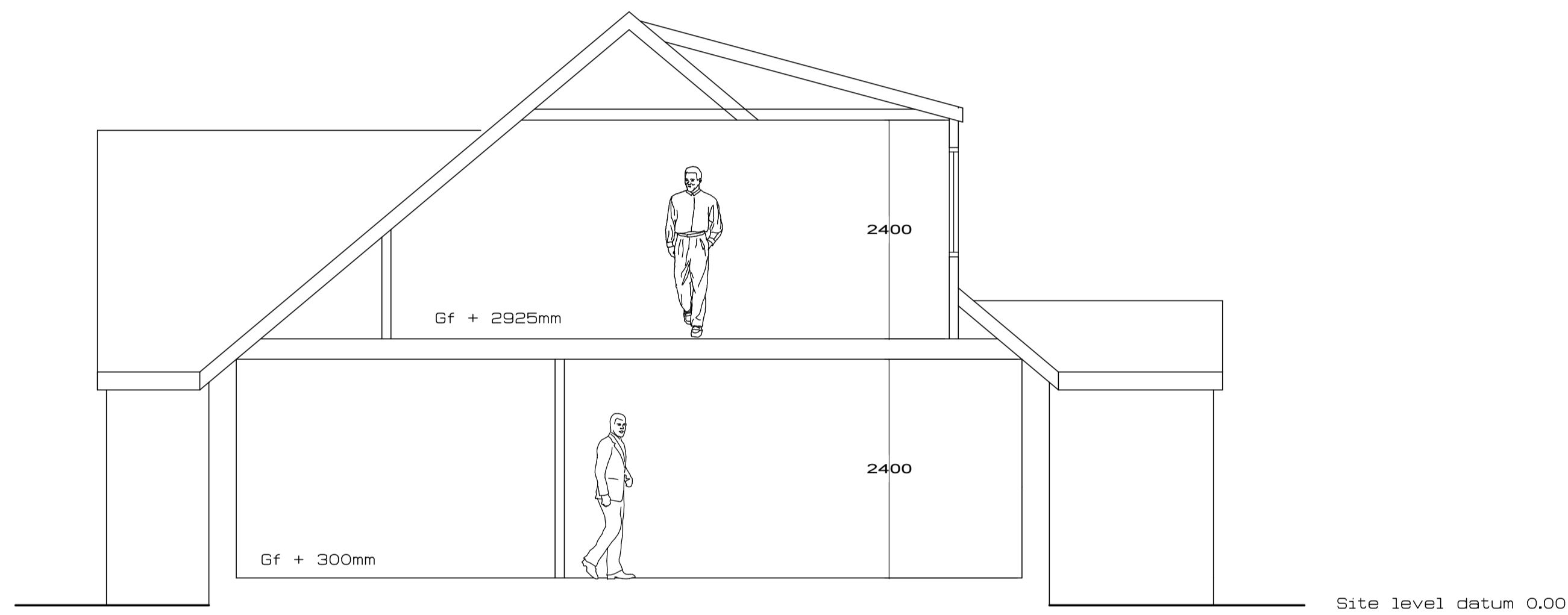
Typical Section
