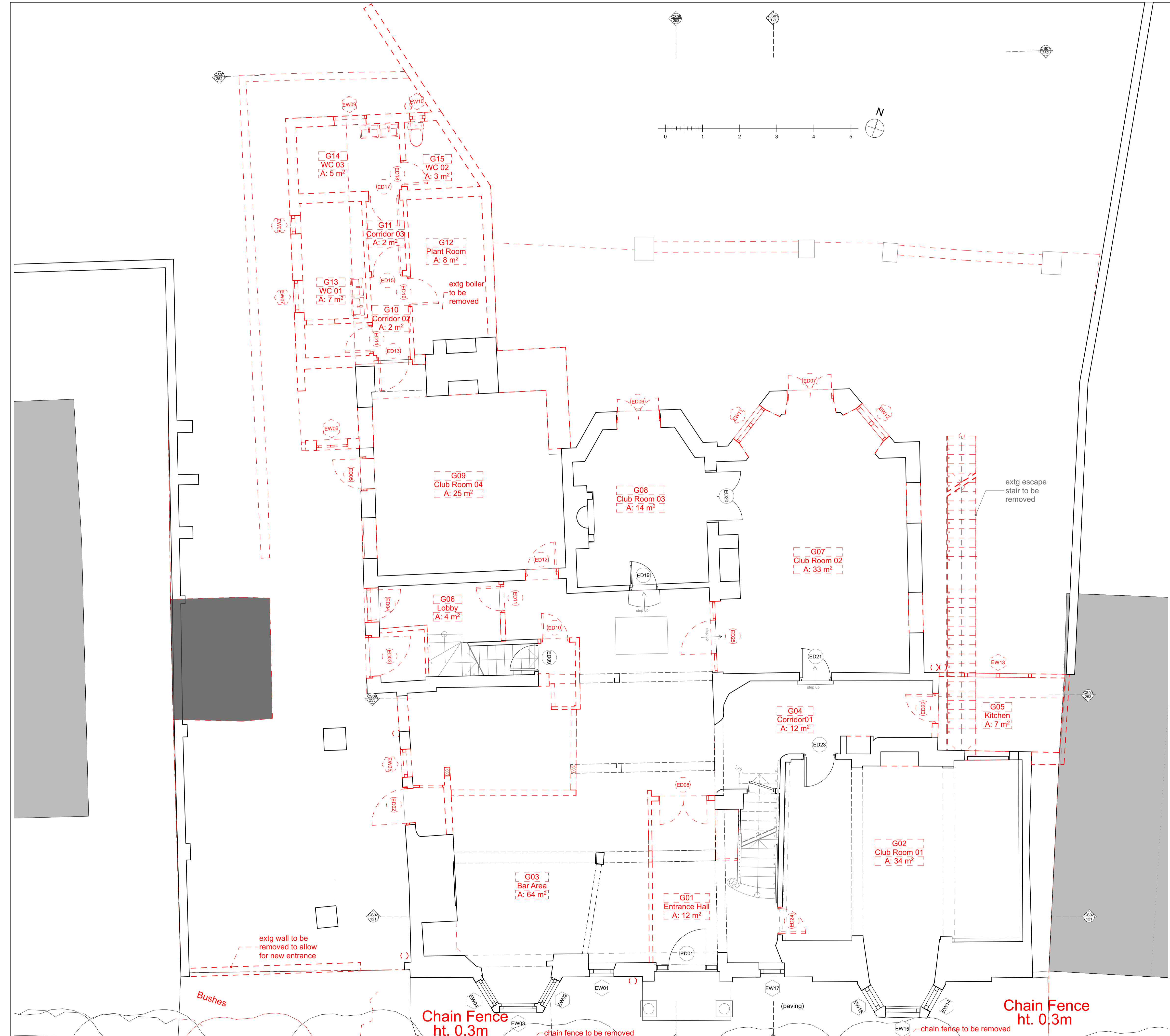
Ground Floor Plan - Removals 1:50
