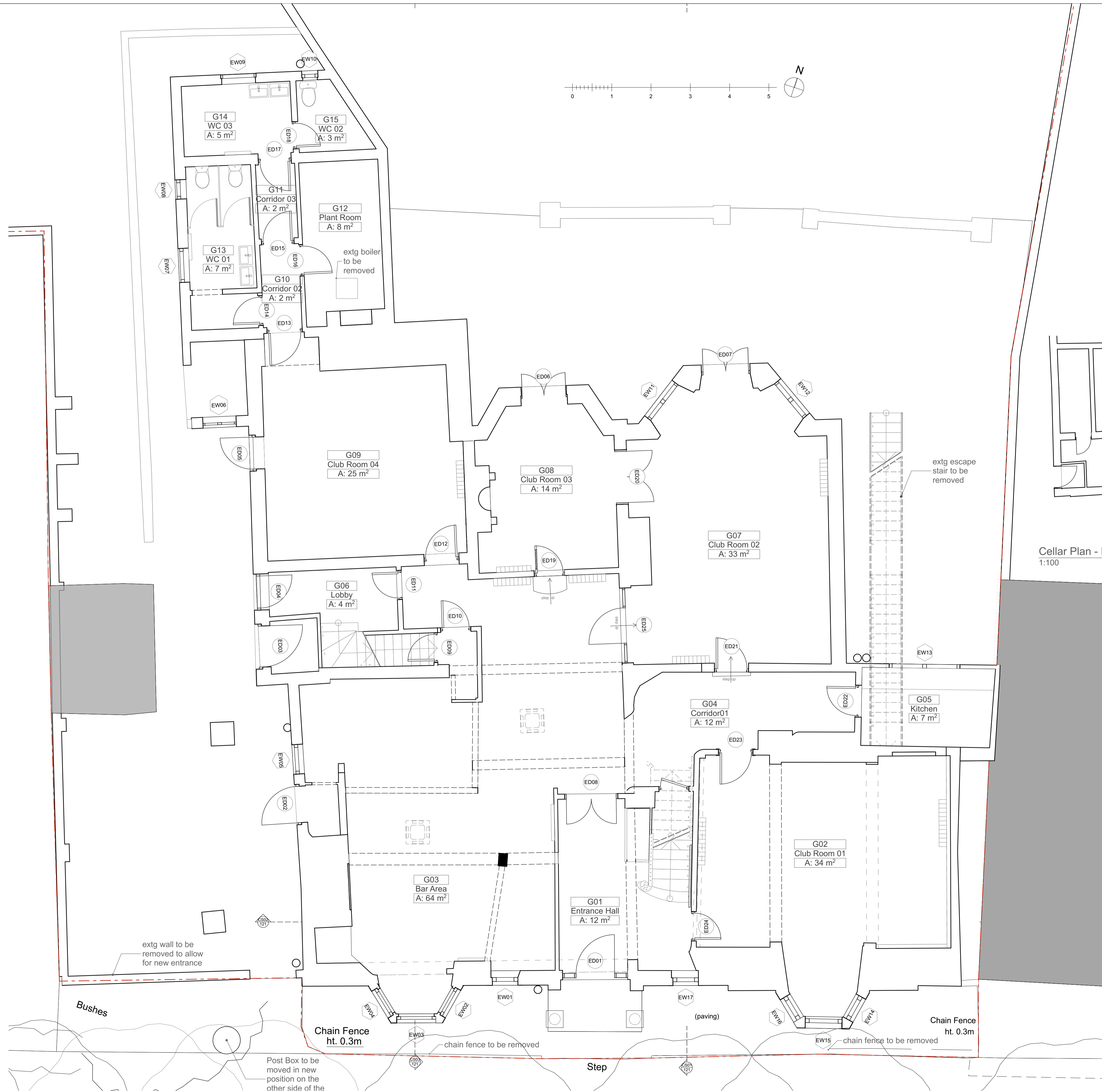
Ground Floor - Existing 1:50
