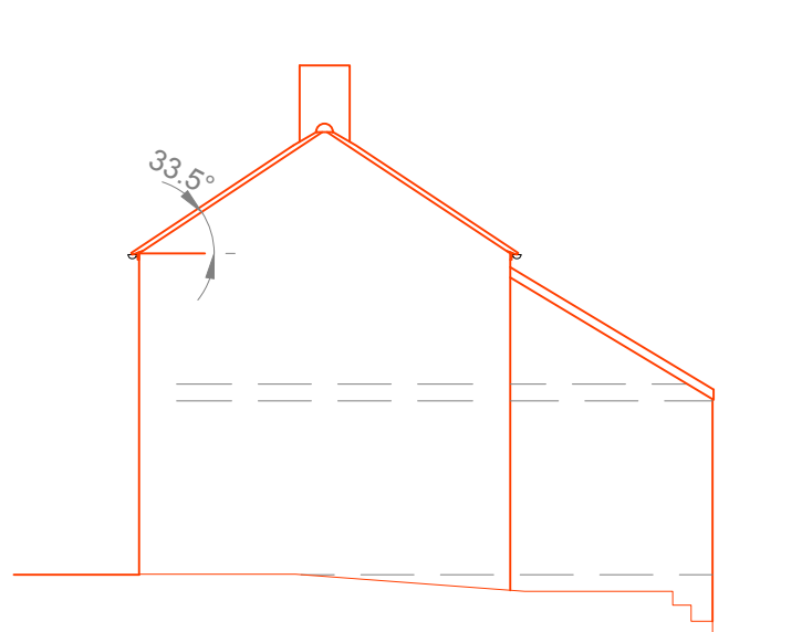
SOUTH ELEVATION
