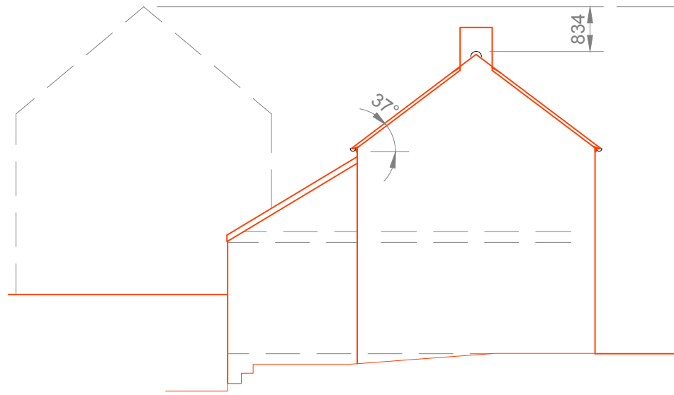
NORTH ELEVATION
