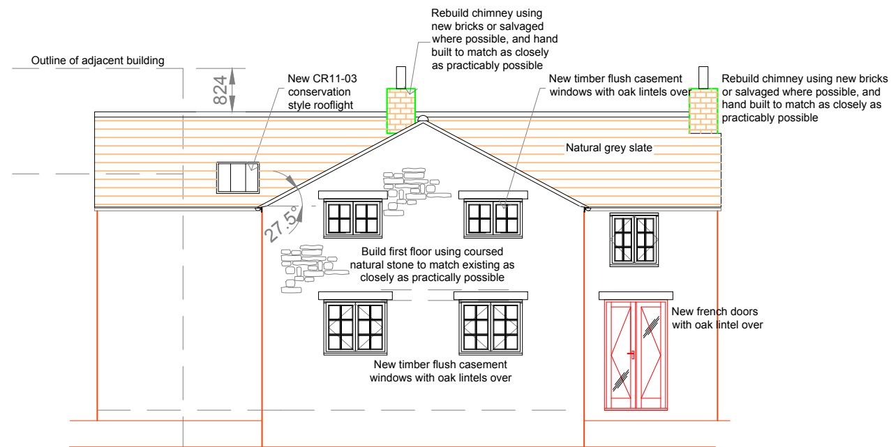
EAST ELEVATION
