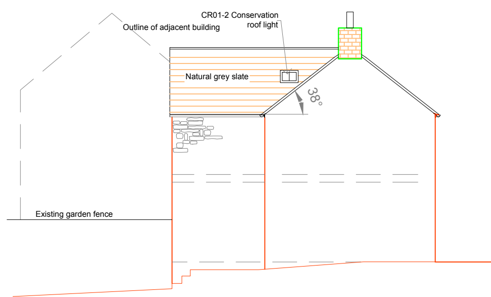
NORTH ELEVATION
