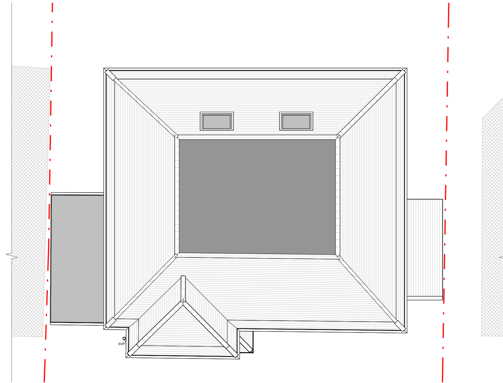
Roof Plan
