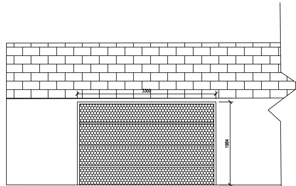
Proposed Door 1:50
