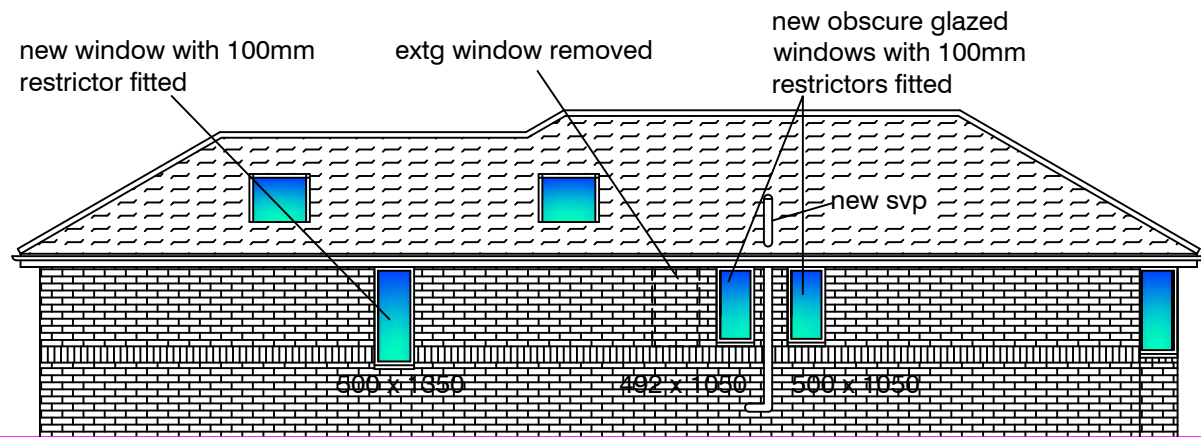
SIDE ELEVATION
