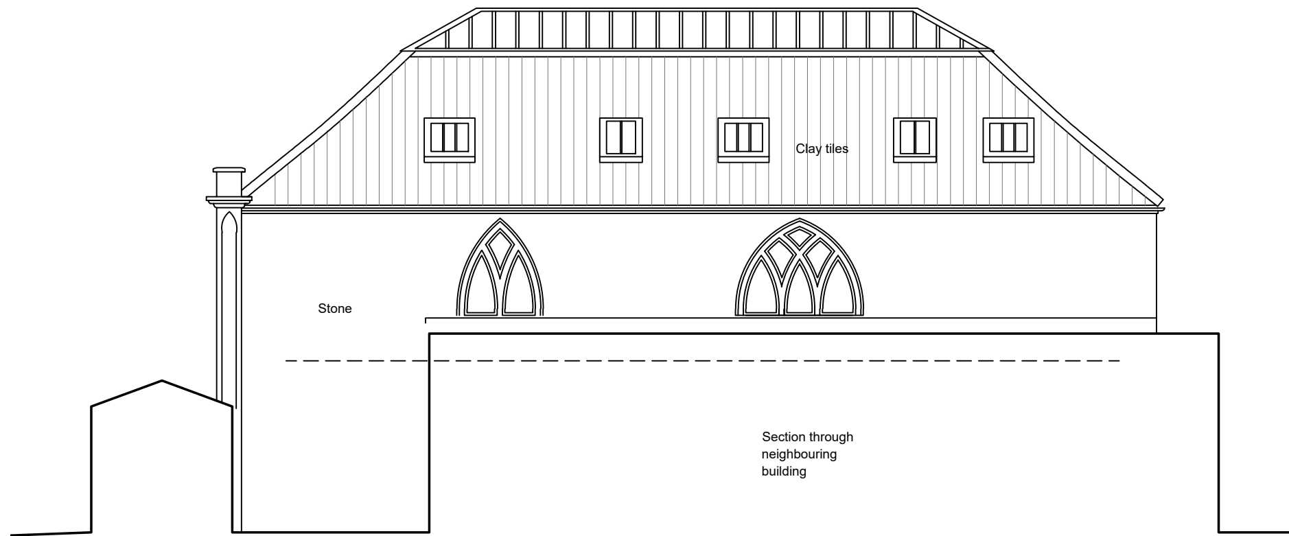
② North 1:100
