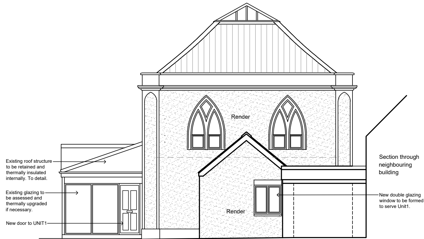
3 East 1:100
