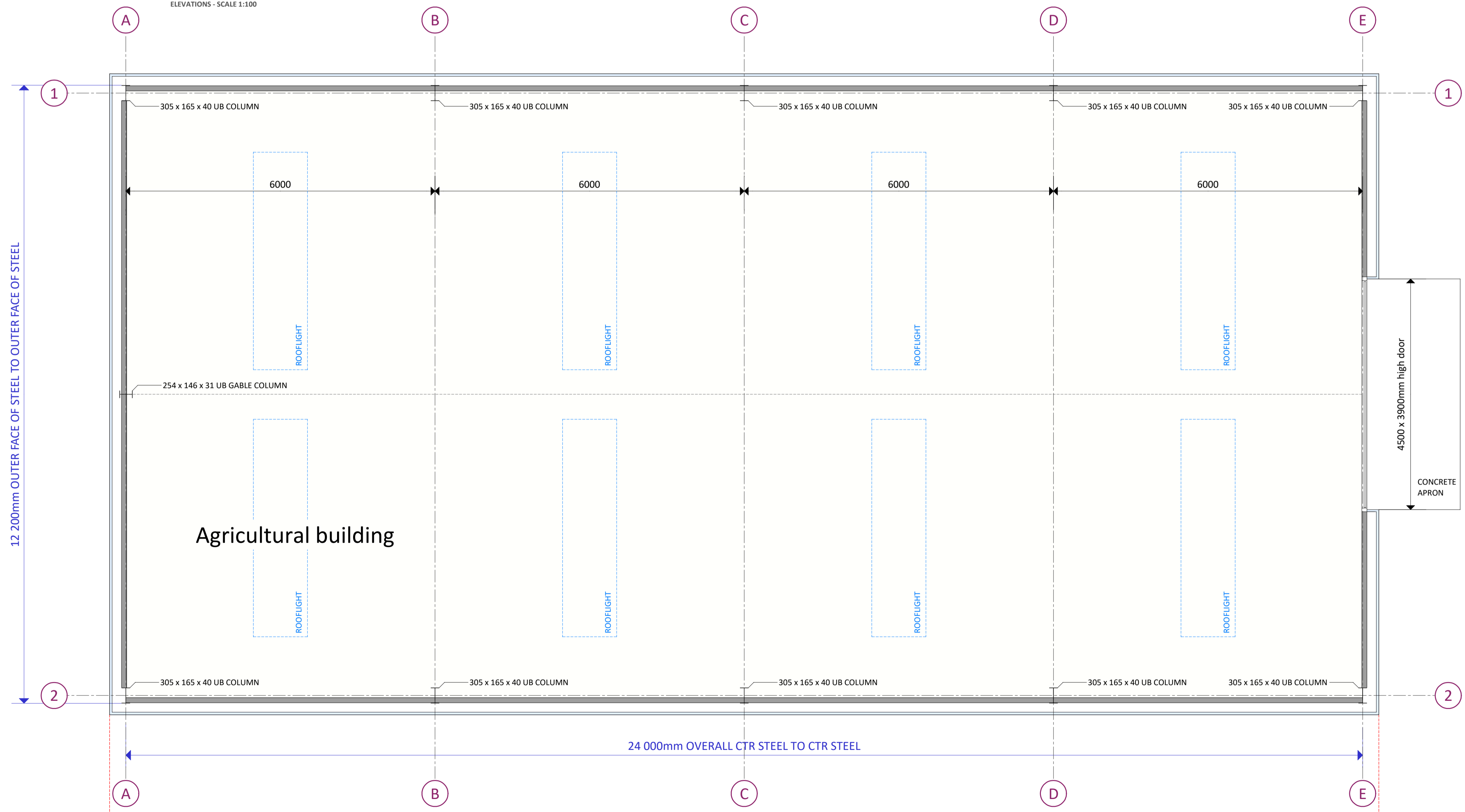
GROUND FLOOR PLAN 0 1 2 3m SCALE 1:50
