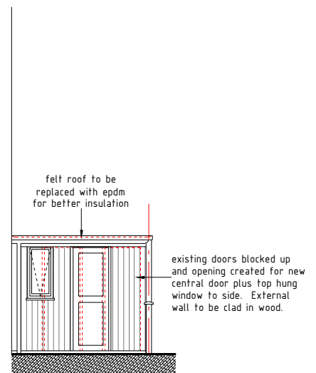
SECTION A-A (as proposed)
