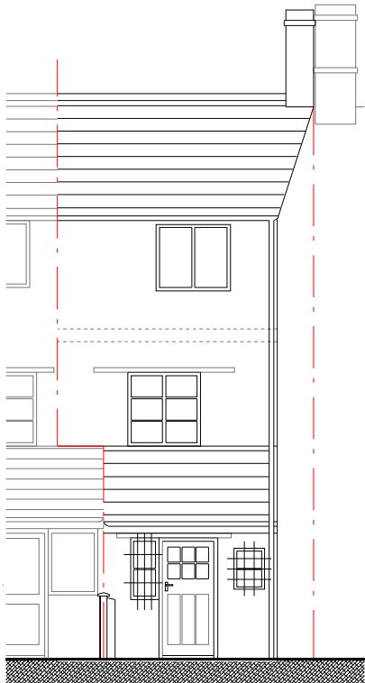
REAR ELEVATION (as existing)
