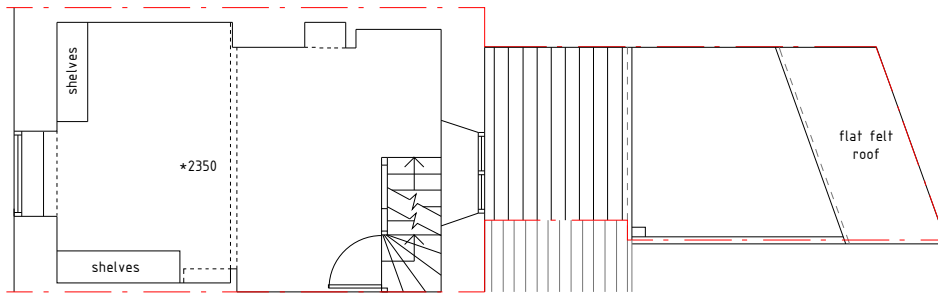
FIRST FLOOR PLAN (as existing)
