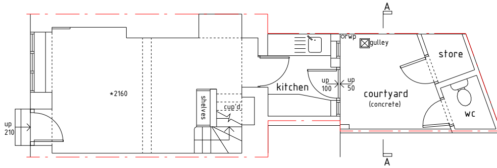
GROUND FLOOR PLAN (as existing)
