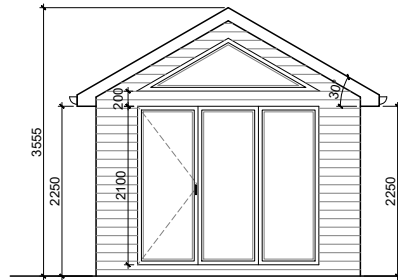
FRONT ELEVATION SCALE 1:100 @A4
