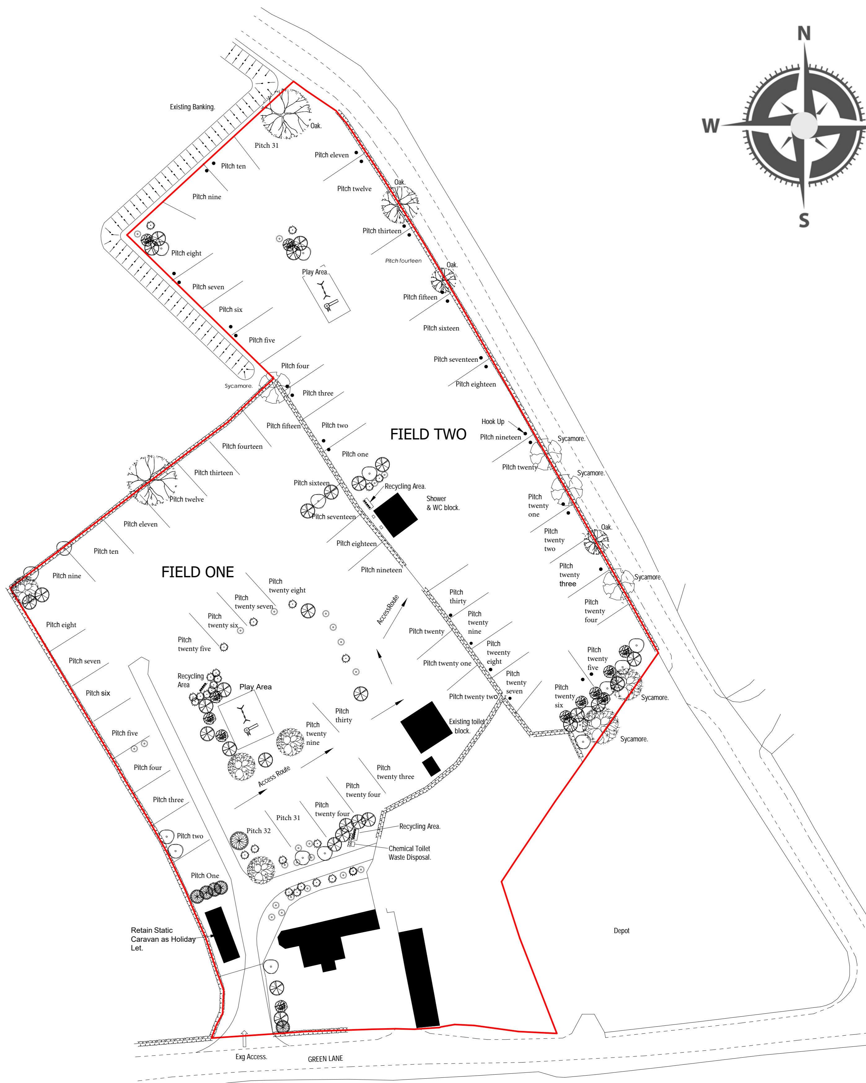
PROPOSED SITE PLAN SCALE 1-500
