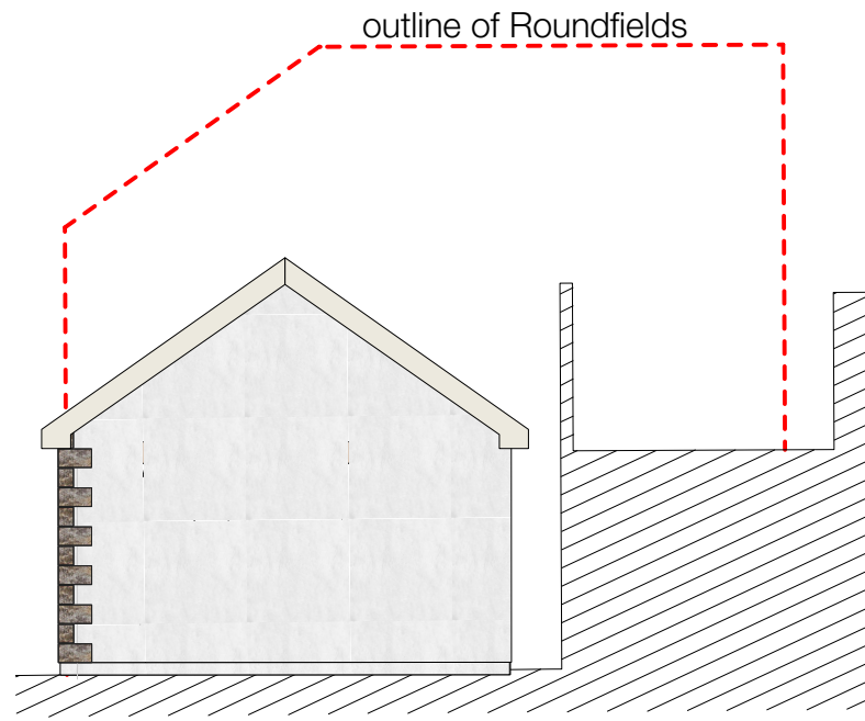
South Elevation SCALE 1:100
