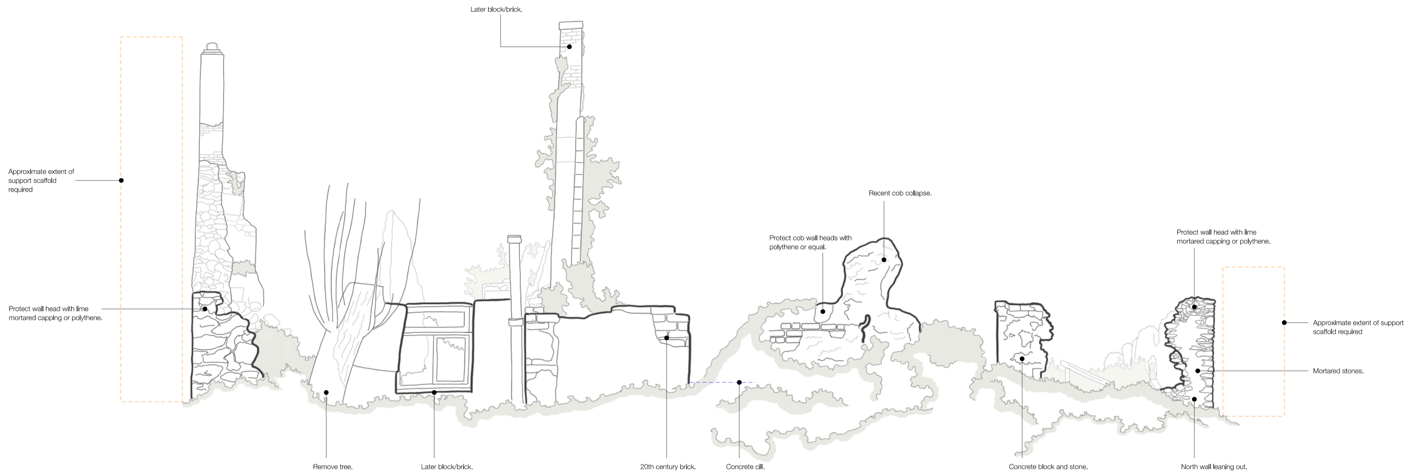
EAST ELEVATION
