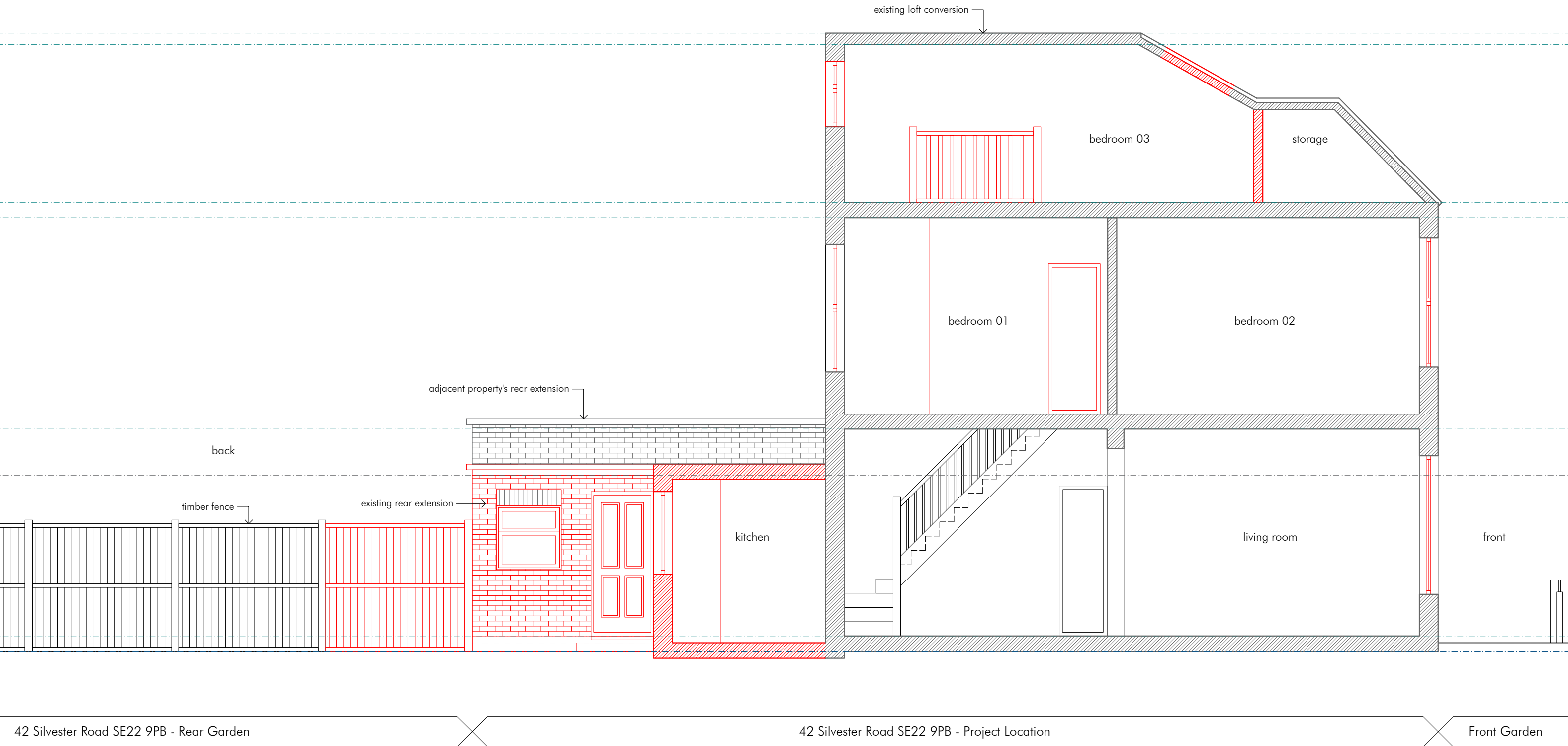
Demolition section A-A
