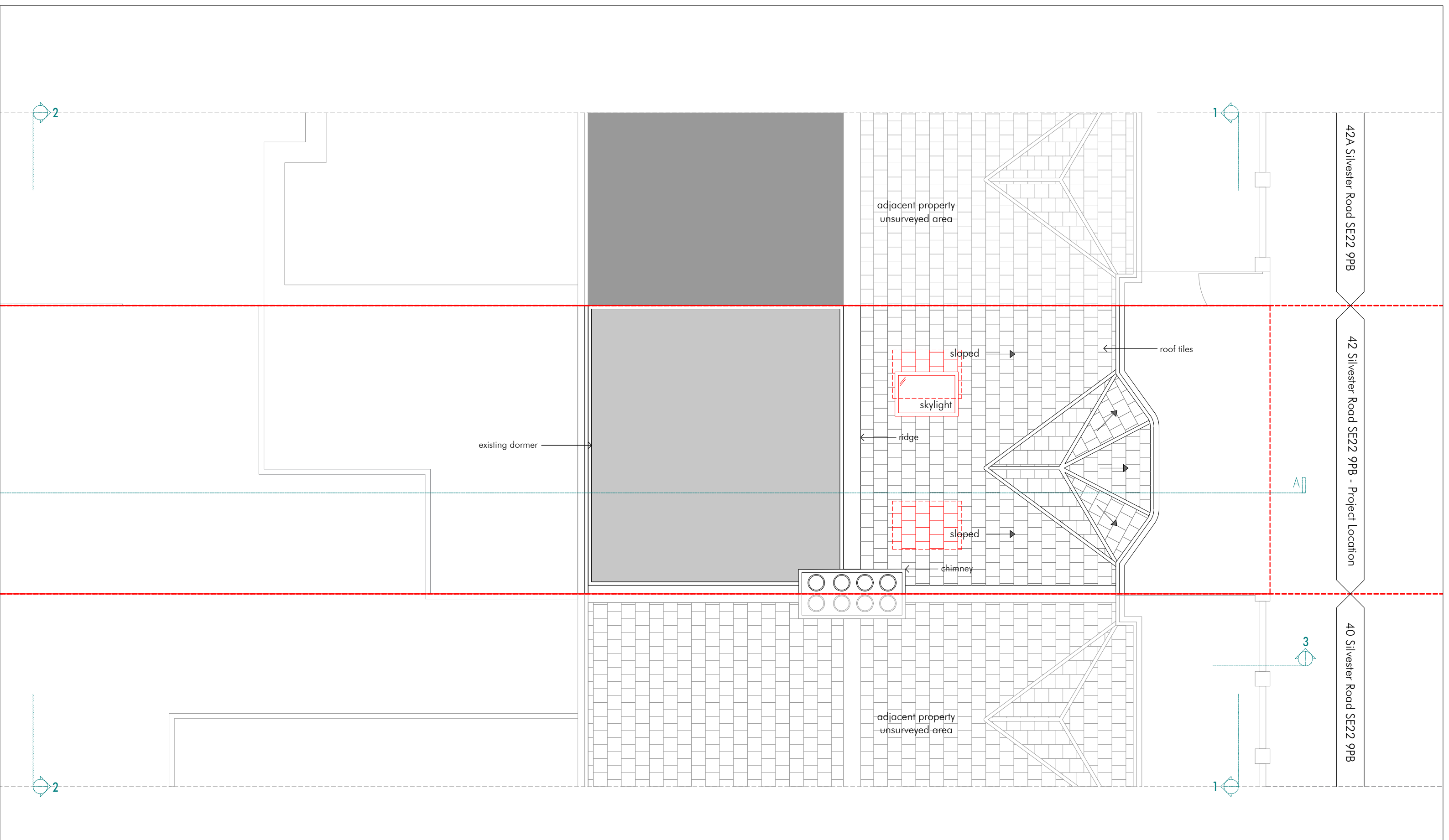
Demolition roof plan
