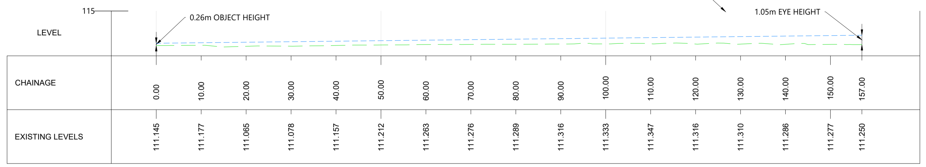
LONGSECTION OF 157m FORWARD VISIBILITY TO SITE ACCESS - SOUTHBOUND 1.5 x SSD (START) SCALE: H 1:500, V 1:250. DATUM: 110.000
