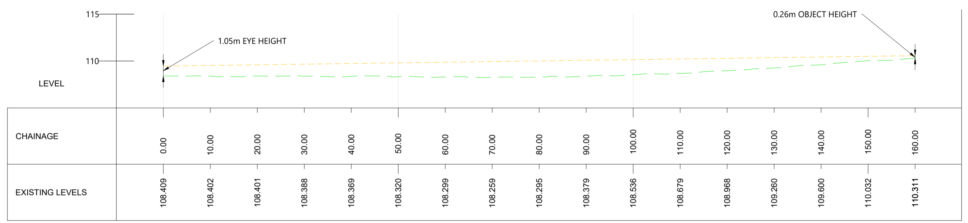
LONGSECTION OF 160m FORWARD VISIBILITY TO SITE ACCESS - NORTHBOUND 1.5 x SSD (MIDDLE) SCALE: H 1:500,V 1:250. DATUM: 105.000
