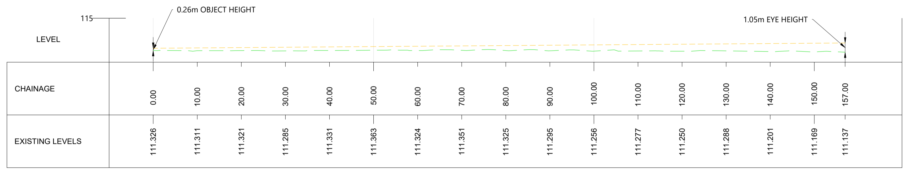
LONGSECTION OF 157m FORWARD VISIBILITY TO SITE ACCESS - SOUTHBOUND 1.5 x SSD (MIDDLE) SCALE: H 1:500, V 1:250. DATUM: 110.000
