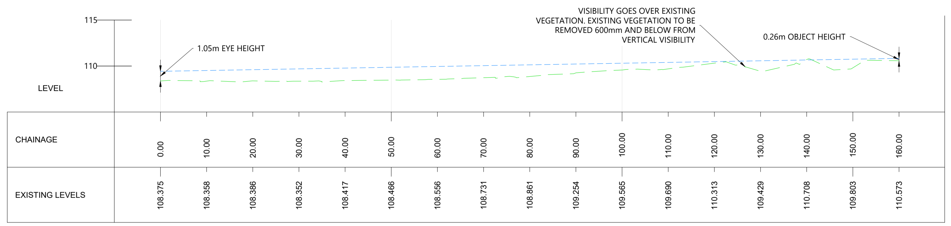
LONGSECTION OF 160m FORWARD VISIBILITY TO SITE ACCESS - NORTHBOUND 1.5 x SSD (START) SCALE: H 1:500,V 1:250. DATUM: 105.000
