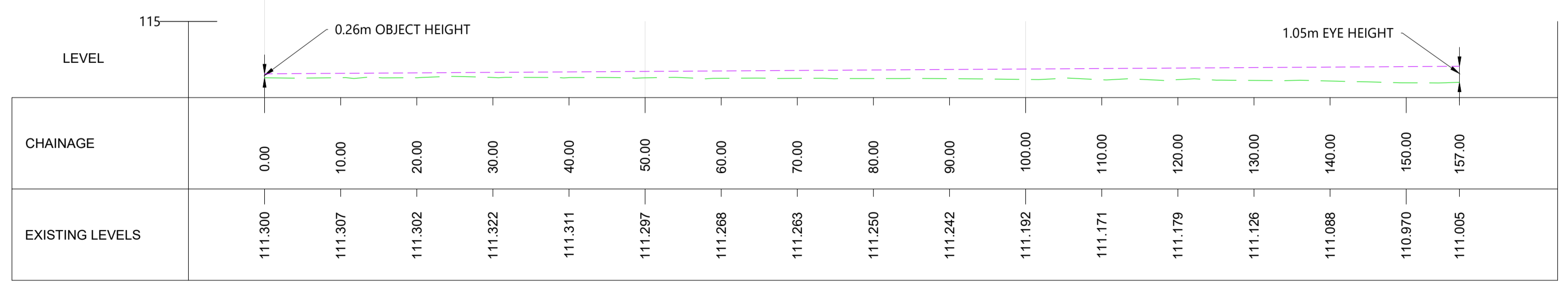
LONGSECTION OF 157m FORWARD VISIBILITY TO SITE ACCESS - SOUTHBOUND 1.5 x SSD (END) SCALE: H 1:500, V 1:250. DATUM: 110.000
