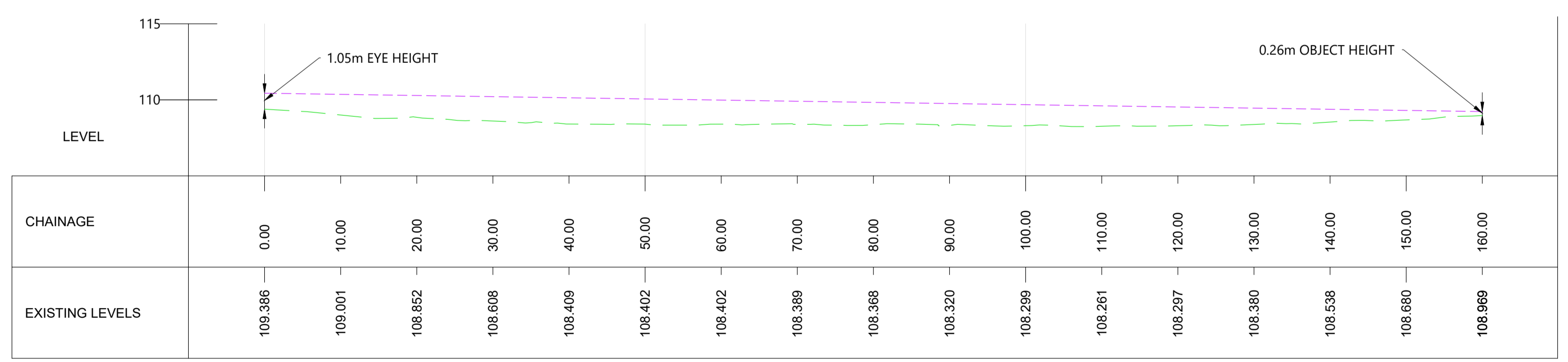
LONGSECTION OF 160m FORWARD VISIBILITY TO SITE ACCESS - NORTHBOUND 1.5 x SSD (END) SCALE: H 1:500,V 1:250. DATUM: 105.000
