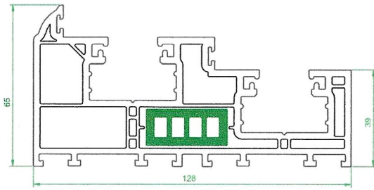
4001 Outer Frame
