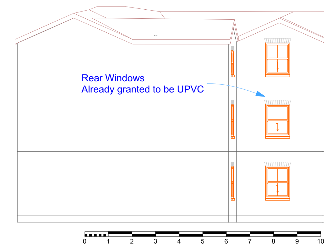
8 South Elevation Proposed 1:100
