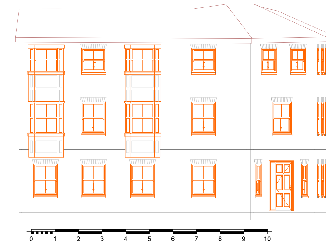
7 North Elevation Proposed 1:100
