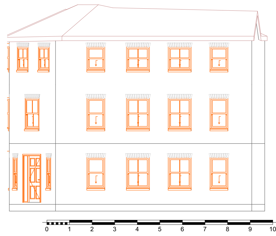
2 West Elevation Existing 1:100
