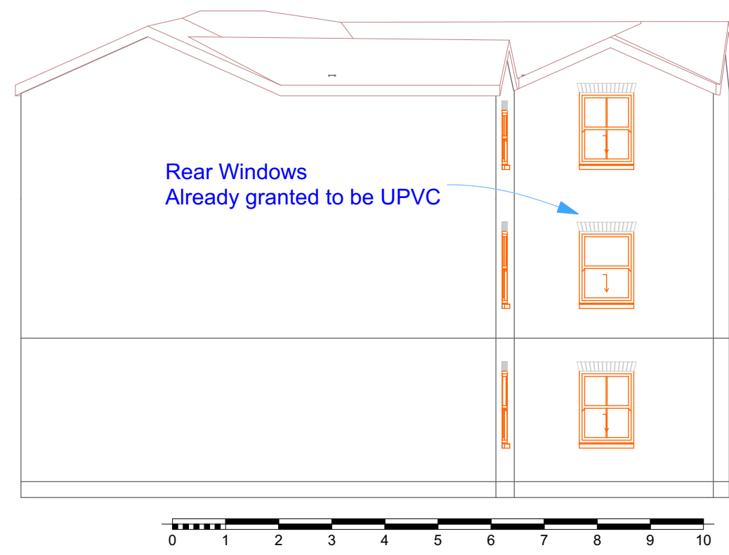
4 South Elevation Existing 1:100
