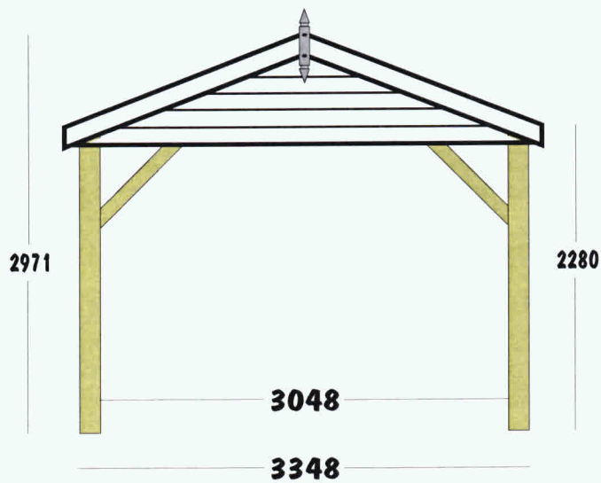
South Elevation
