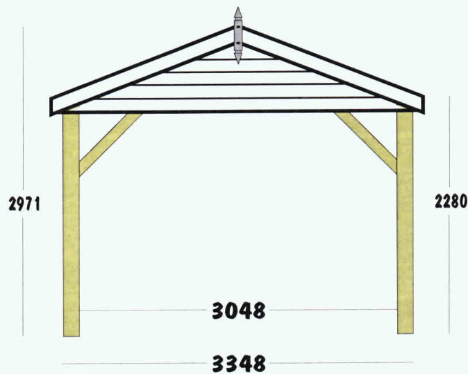
North Elevation
