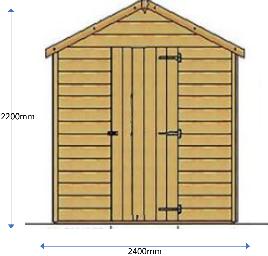
CURRENT FRONT ELEVATION
