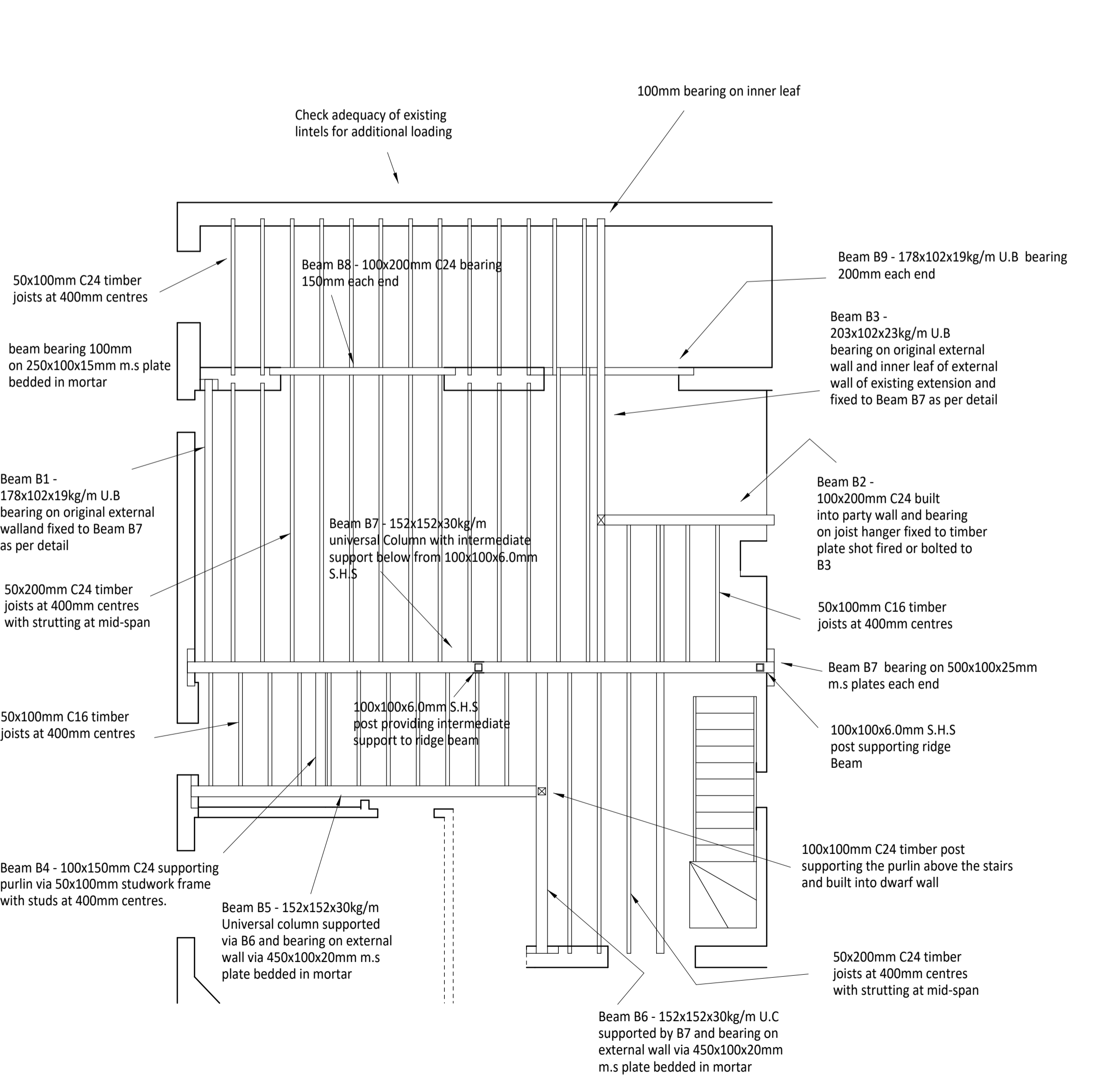
STRUCTURAL LAYOUT
