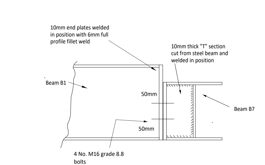
Connection detail Beam B1 & B3 to B7
