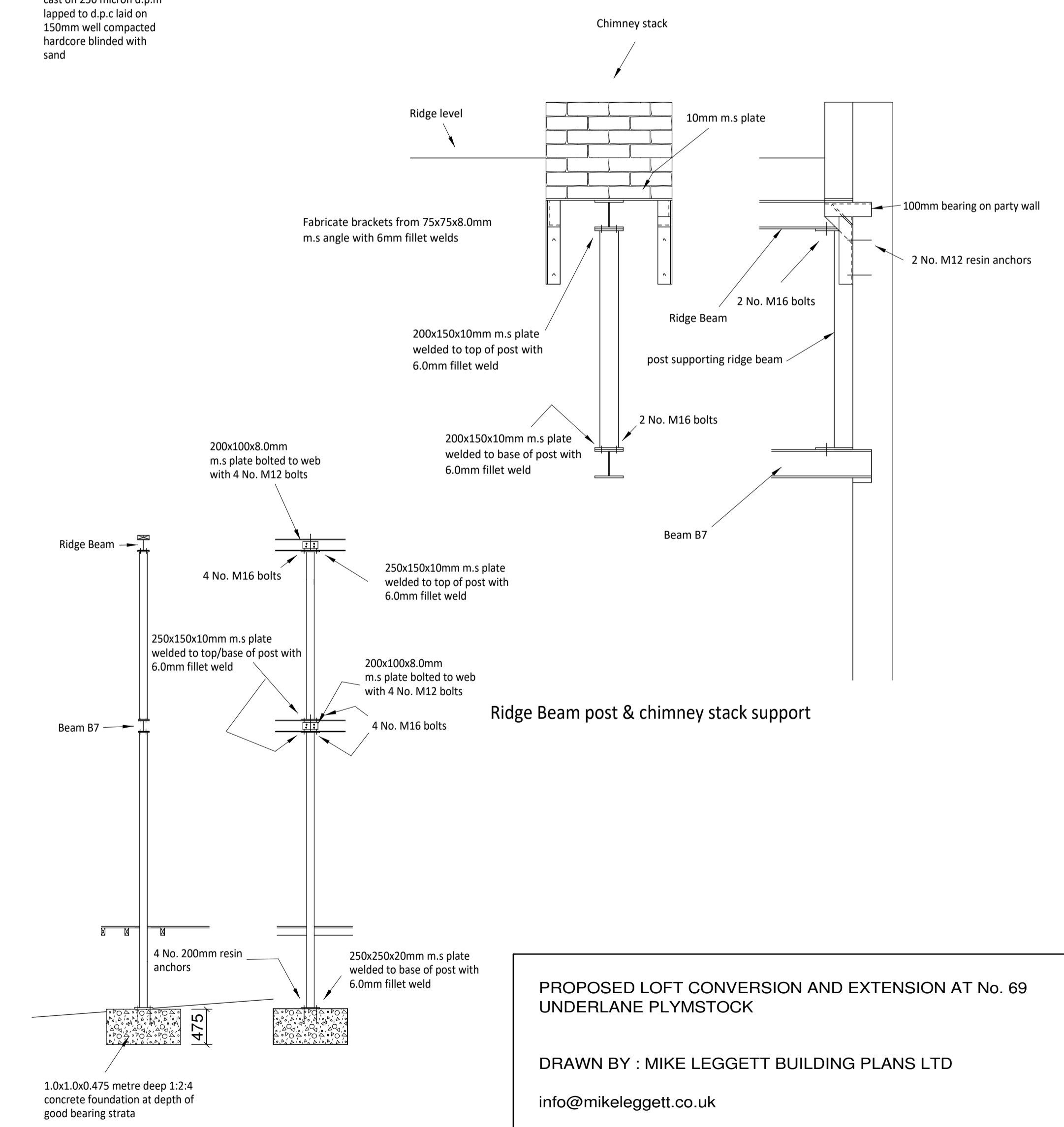
Posts providing intermediate support to ridge beam and support to Beam B7
