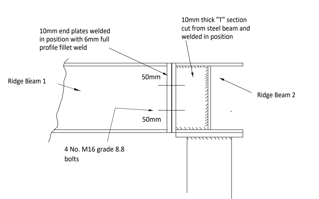
Ridge Beam Connection Detail
