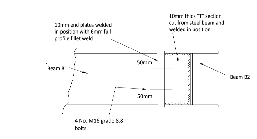
Connection detail Beam B5 to B6 & B6 to B7
