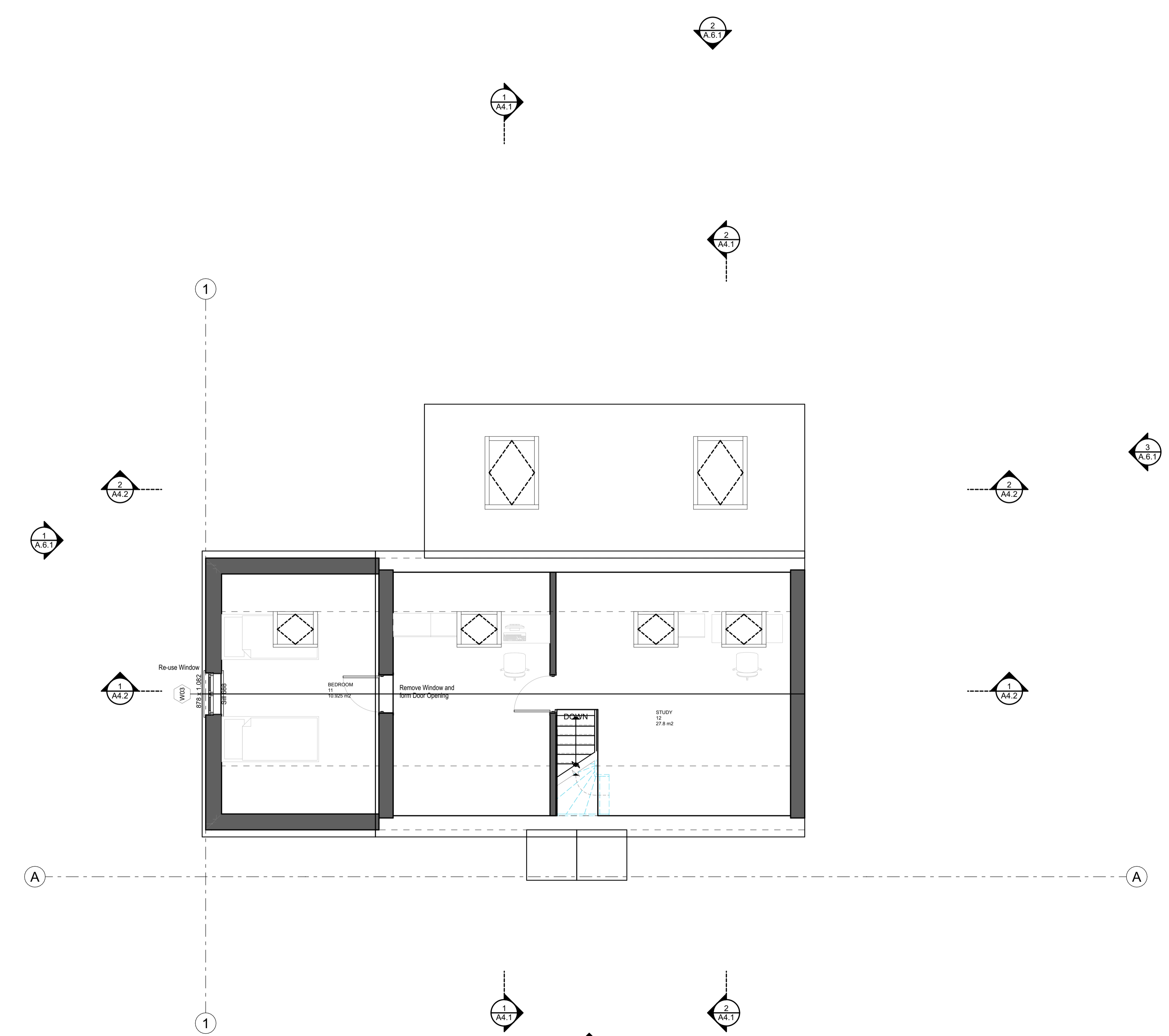
1 2. Loft Conversion 1:50
